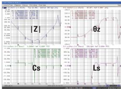
PDN measurement with S-parameter port 1-2 shunt-thru method (100 Hz to 1 GHz)
