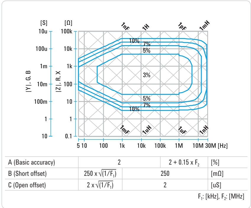
Figure 5. Impedance measurement accuracy (SPD), Gain-phase series-thru method (T: 50 Ω 0 dB, R: 1 MΩ 0 dB).
