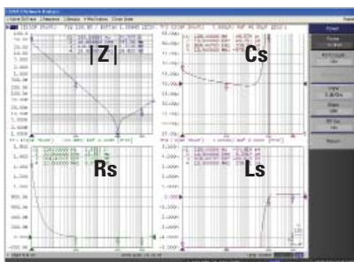
MLCC measurement with Gain-phase shunt-thru method (100 Hz to 30 MHz)
