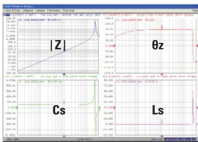
RF inductor measurement with reflection method (1 MHz to 3 GHz)
