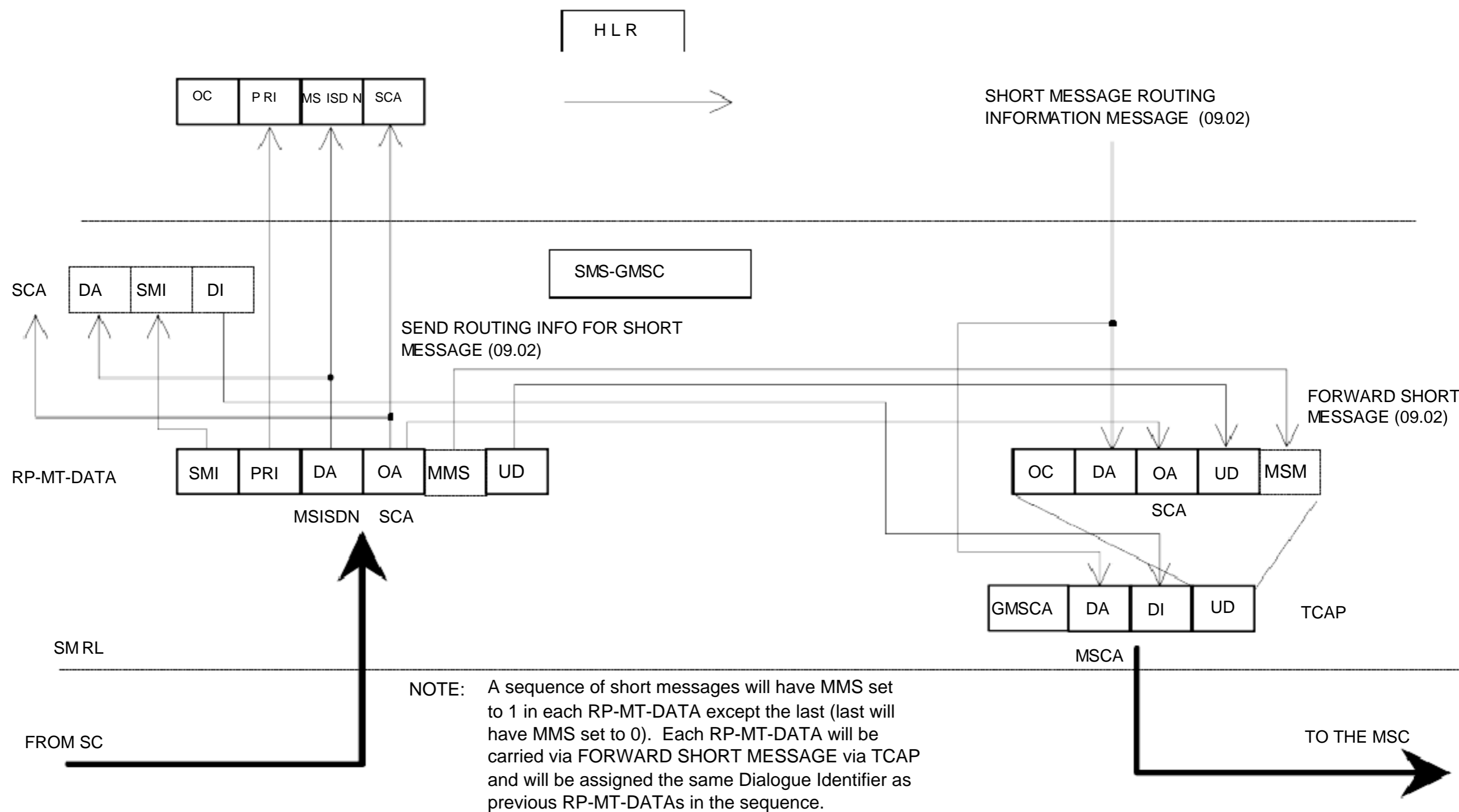
Figure 1.2: Mobile terminated short message
