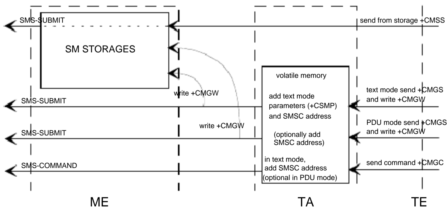
Figure 4: Message service send and write procedures
