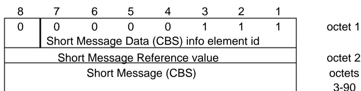
Figure 2.5.9/GSM 07.05: Short Message Data (CBS) information element
