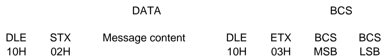
Figure 2.2.1/GSM 07.05: Format of DTE/DCE interface messages
