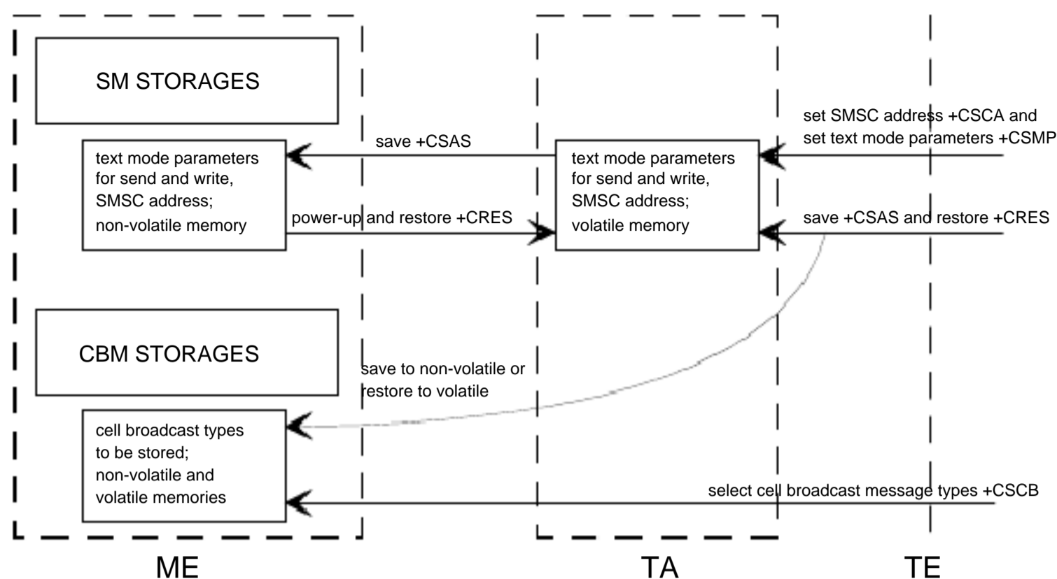
Figure 1: Message service parameter procedures
