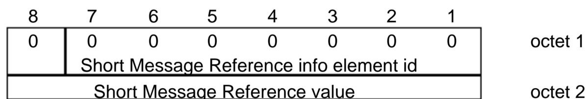
Figure 2.5.2/GSM 07.05: Short Message Reference information element
