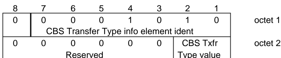
Figure 2.5.12/GSM 07.05: CBS Transfer Type information element
