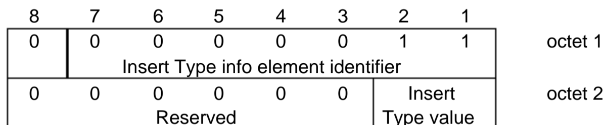
Figure 2.5.5/GSM 07.05: Insert Type information element
