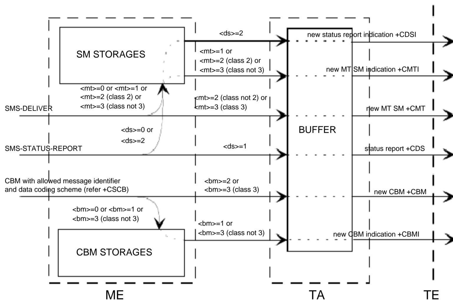
Figure 3: Message receiving procedures
