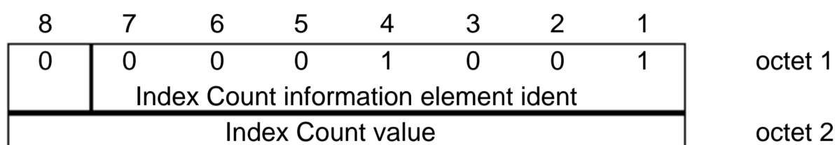
Figure 2.5.11/GSM 07.05: Index Count information element
