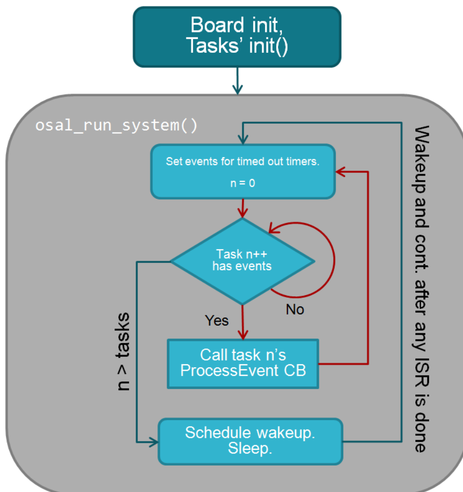
Figure 5: OSAL task loop
