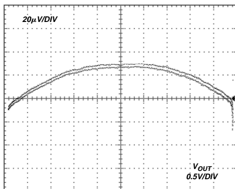
Figure 26. Gain Nonlinearity, V_S = \pm 2.5\text{ V} , G = 5 (4 ppm/DIV) 增益非线性
