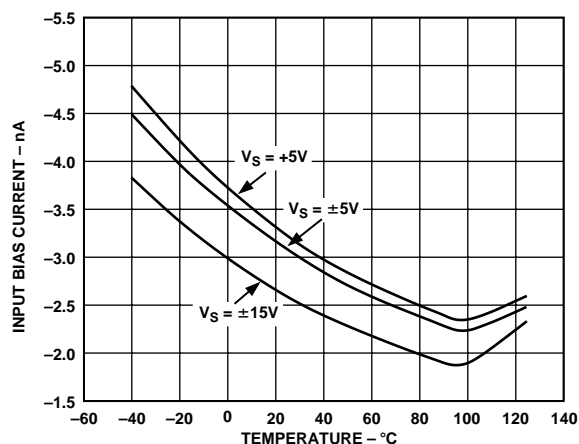
Figure 5. Input Bias Current vs. Temperature 输入偏置电流与温度的关系
