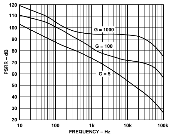
Figure 11. Positive PSRR vs. Frequency, \pm 5 V 正电源抑制比与频率的关系
