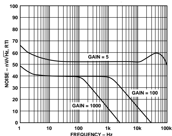
Figure 2. Voltage Noise Spectral Density vs. Frequency 电压噪声谱密度与频率的关系
