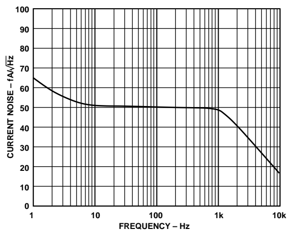
Figure 3. Current Noise Spectral Density vs. Frequency 电流噪声谱密度与频率的关系
