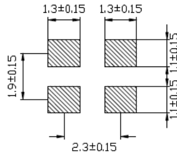
LAND PATTERN<REFERENCE>
