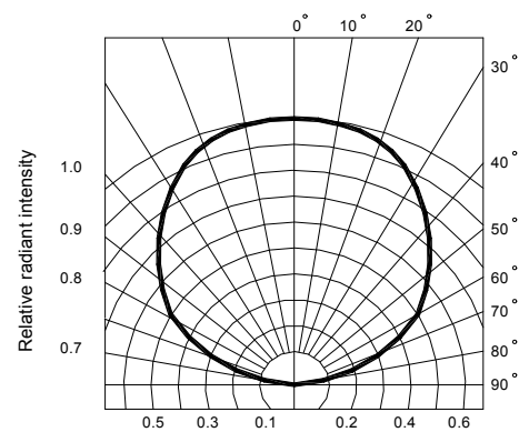
Fig.6 Radiation diagram
