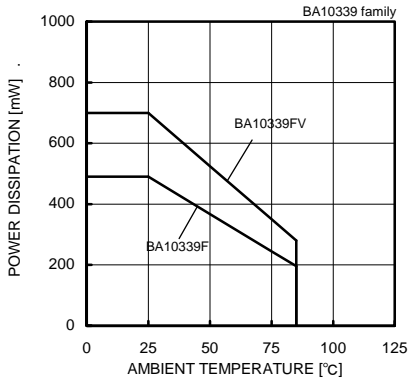
Fig.44 Derating Curve
