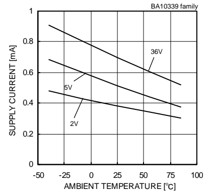
Fig.46 Supply Current - Ambient Temperature
