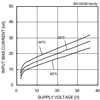
Fig.53 Input Bias Current - Supply Voltage
