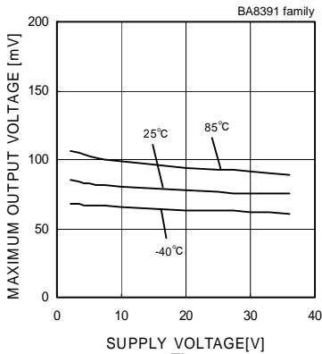
Fig.4 Output Saturation Voltage - Supply Voltage (IOL=4[mA])
