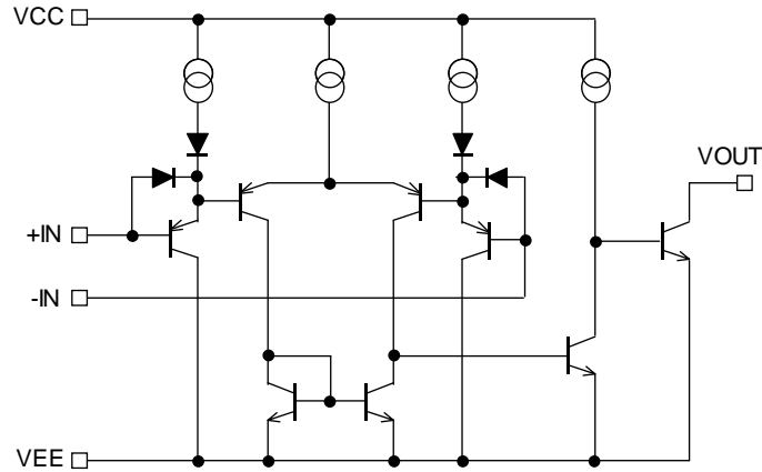
Fig.110 Schematic Diagram (one channel only)
