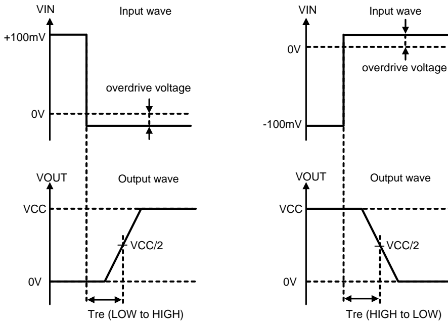
Fig.113 Response Time
