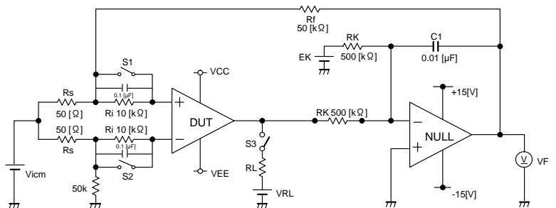
Fig.111 Test circuit1 (one channel only)
