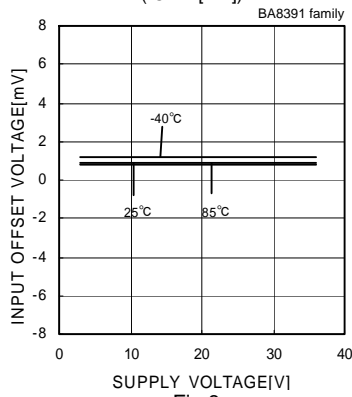
Fig.8 Input Offset Voltage - Supply Voltage
