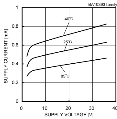
Fig.25 Supply Current - Supply Voltage
