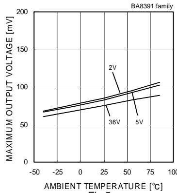
Fig.5 Output Saturation Voltage - Ambient Temperature (IOL=4[mA])
