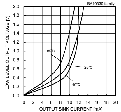
Fig.49 Low Level Output Voltage - Output Sink Current (VCC=5[V])
