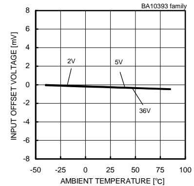
Fig.32 Input Offset Voltage - Ambient Temperature
