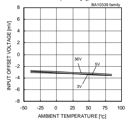
Fig.52 Input Offset Voltage - Ambient Temperature
