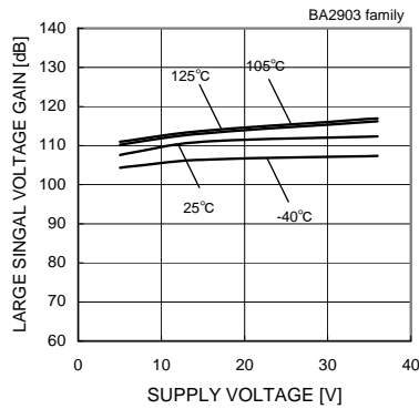
Fig.77 Large Signal Voltage Gain - Supply Voltage
