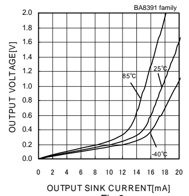
Fig.6 Low Level Output Voltage - Output Sink Current (VCC=5[V])
