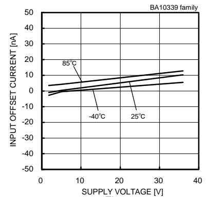
Fig.55 Input Offset Current - Supply Voltage
