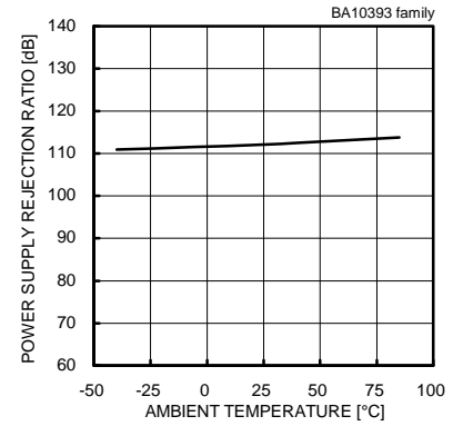
Fig.41 Power Supply Rejection Ratio - Ambient Temperature
