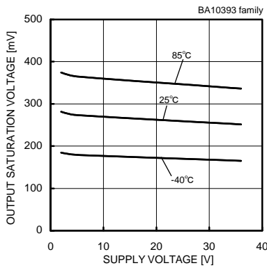
Fig.27 Output Saturation Voltage - Supply Voltage (IOL=4[mA])
