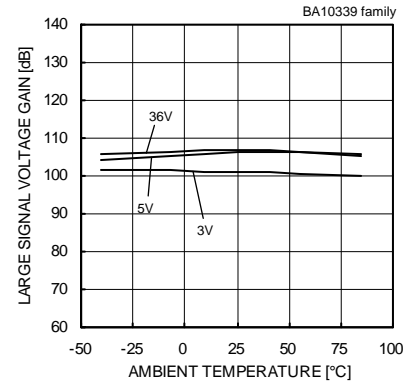
Fig.58 Large Signal Voltage Gain - Ambient Temperature
