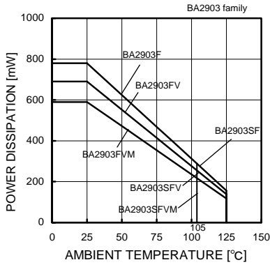
Fig.64 Derating Curve
