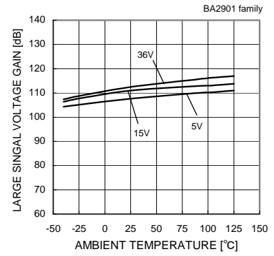
Fig.101 Large Signal Voltage Gain - Ambient Temperature
