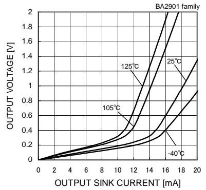
Fig.92 Low Level Output Voltage - Output Sink Current (VCC=5[V])
