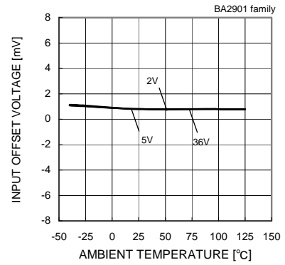
Fig.95 Input Offset Voltage - Ambient Temperature
