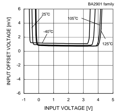
Fig.104 Input Offset Voltage - Input Voltage (VCC=5V)
