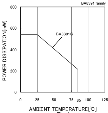
Fig.1 Derating Curve
