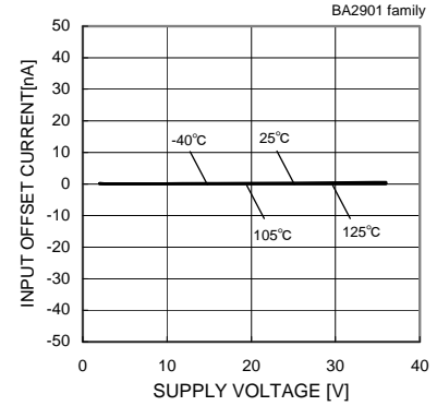
Fig.98 Input Offset Current - Supply Voltage
