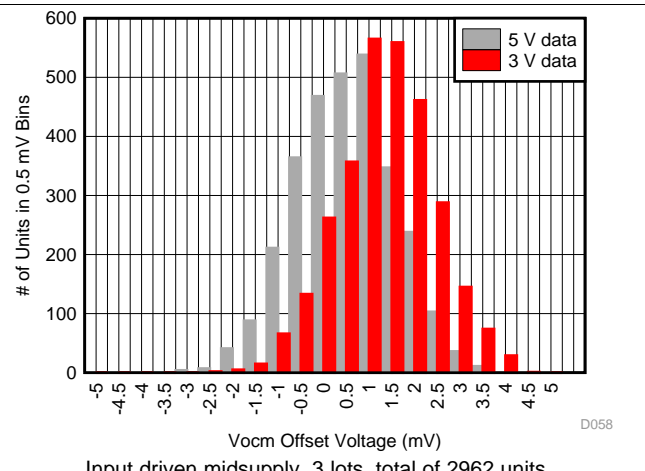
Figure 58. Common-Mode Output Offset from Driven Vocm
