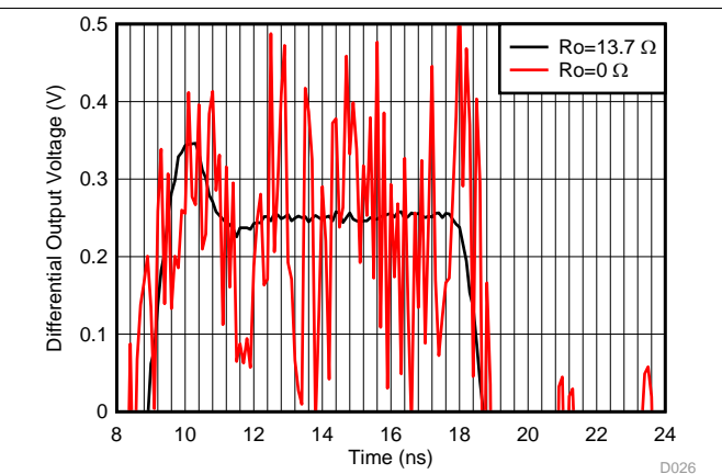
500-mV PP output into 22-pF load, see Figure 71 with V_{s+} = 3\text{ V} and V_{ocm} = 1.5\text{ V}
