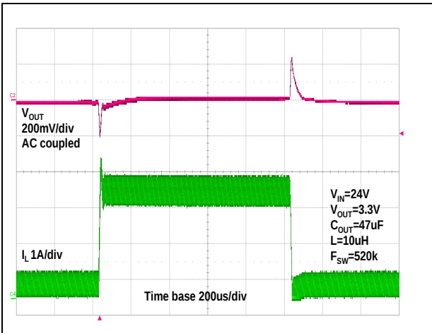
Figure 30. Load transient: from 0.4 A to 2 A
