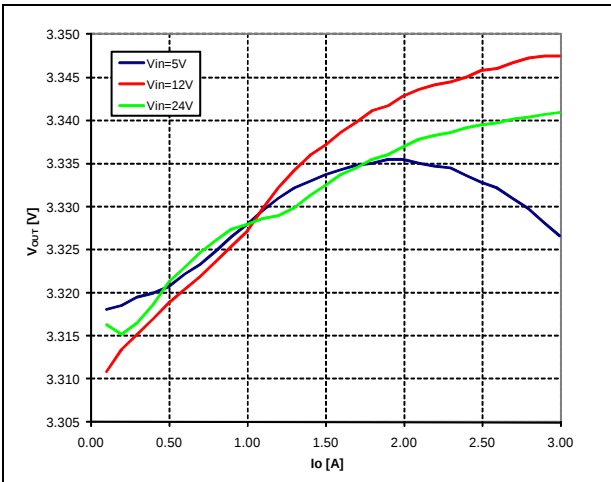
Figure 28. Load regulation
