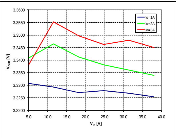
Figure 29. Line regulation
