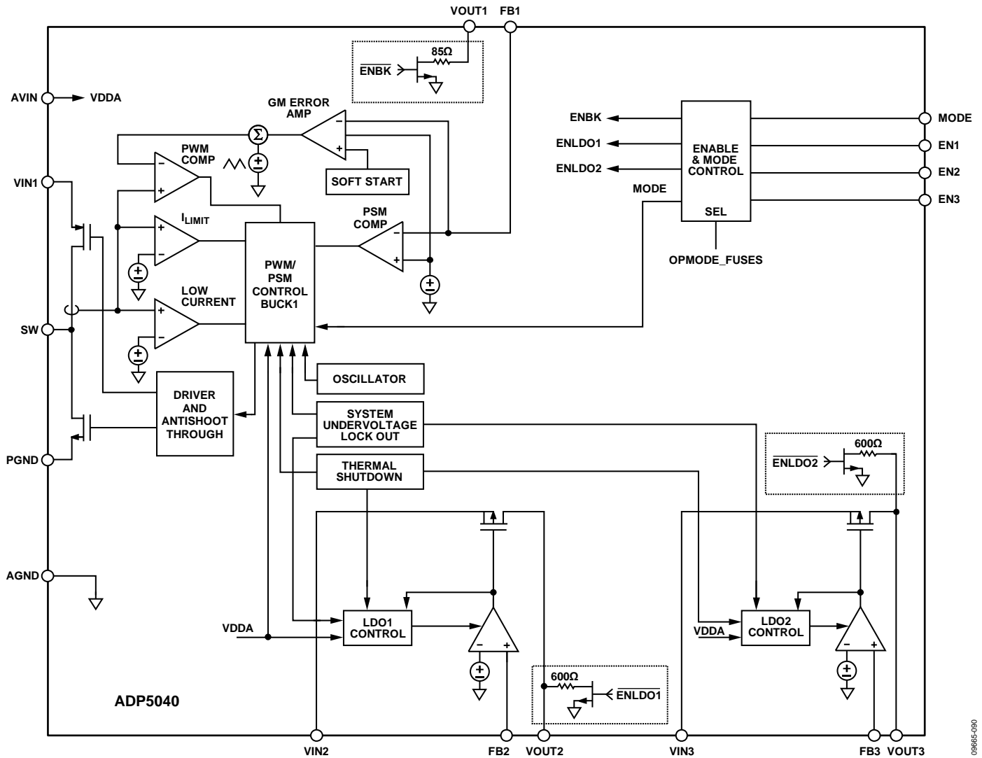
Figure 101. Functional Block Diagram
