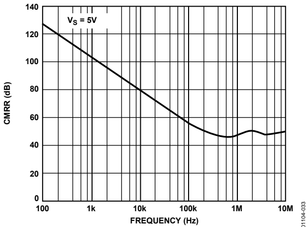
Figure 33. CMRR vs. Frequency at 5 V
