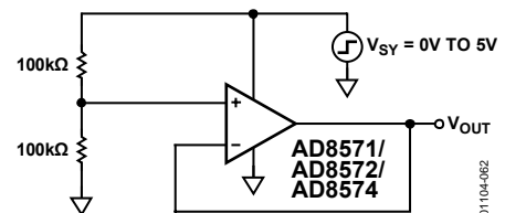
Figure 62. AD857x Test Circuit for Turn-On Time
