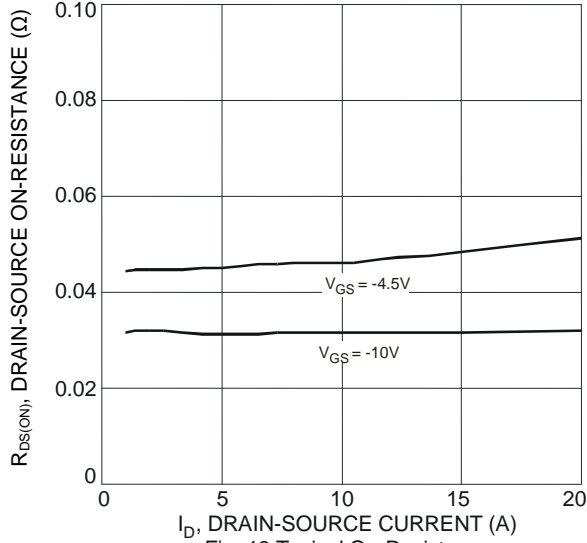
Fig. 13 Typical On-Resistance vs. Drain Current and Gate Voltage
