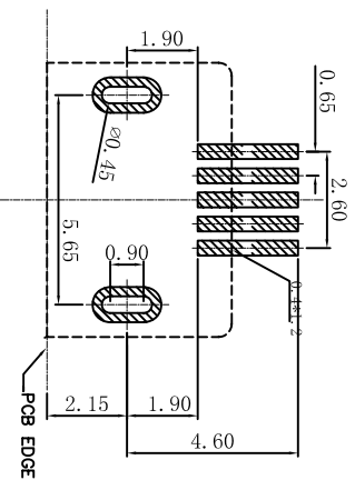
P. C. B LAYOUT
