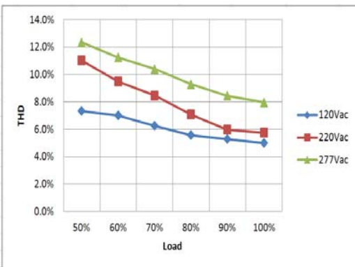
THD Curve(Ref.)
