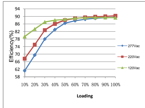
Efficiency VS. Load Curve(Ref.)
