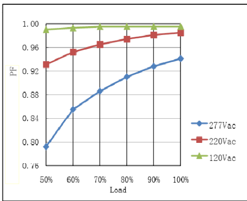
Power Factor VS. Load Curve
