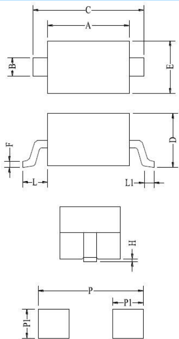
Land Pattern
