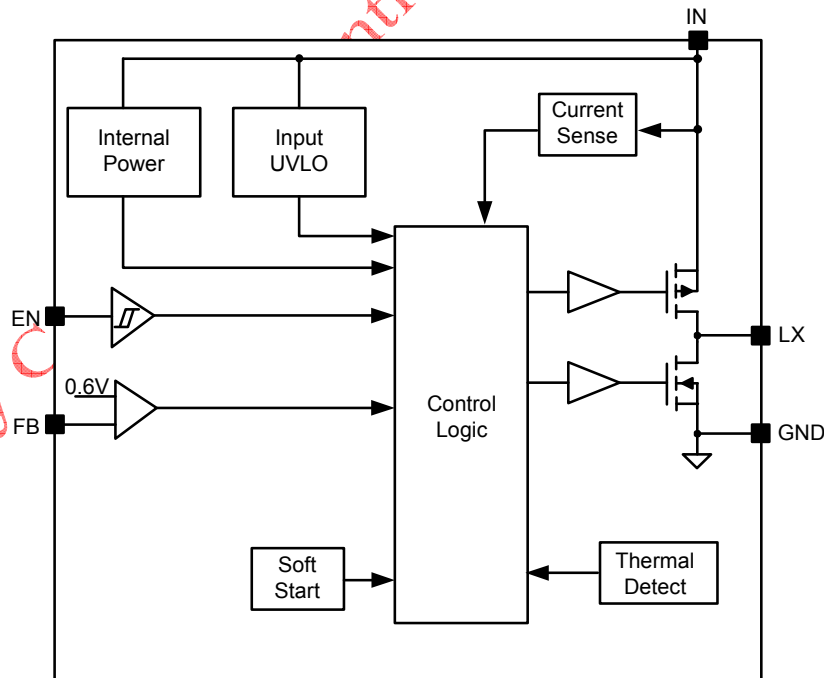
Figure2. Block Diagram
