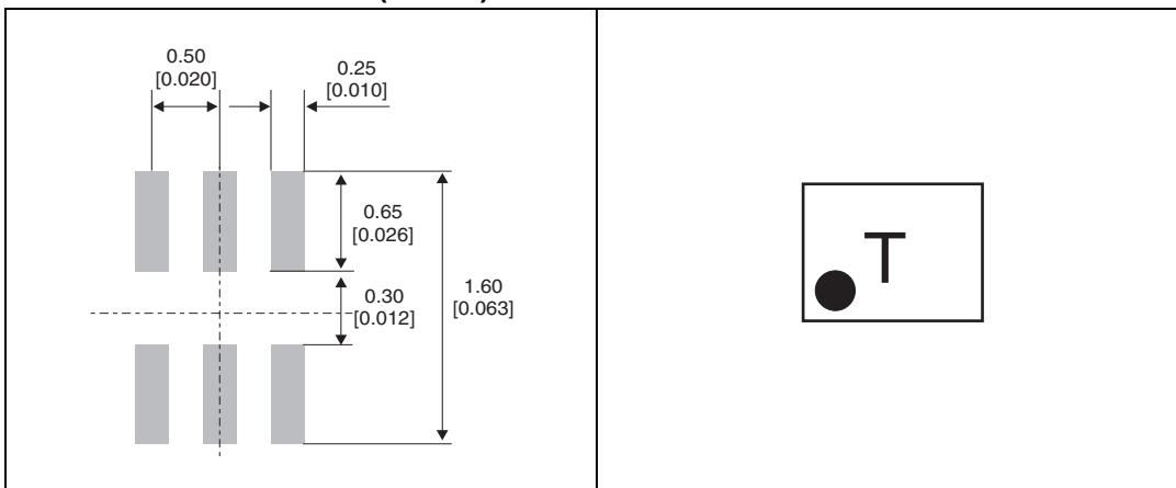
Figure 9. Footprint recommendations dimensions in mm (inches)
