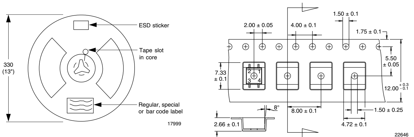
Fig. 12 - Tape and Reel Shipping Medium, 2000 units per reel
