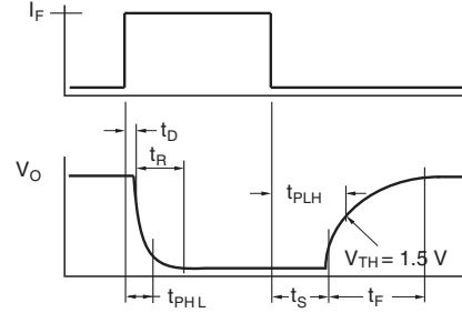
Fig. 6 - Switching Timing
