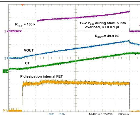
Figure 22. Power Dissipation During 12-V Startup into 15 \Omega , 140 \mu F
