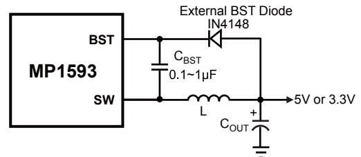
Figure 4—Add Optional External Bootstrap Diode to Enhance Efficiency
