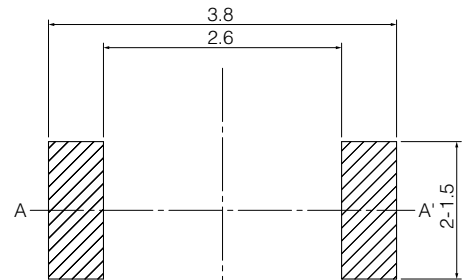
Land pattern plan
