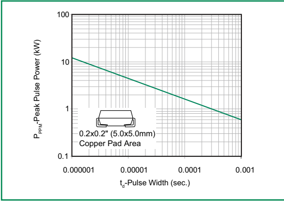
Figure 1 - Peak Pulse Power Rating
