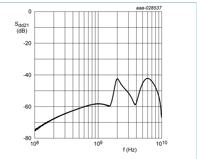
Fig. 2. Differential crosstalk; typical values
