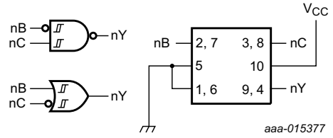
Fig 6. 2-input NAND gate with input B inverted or 2-input OR gate with inverted C input
