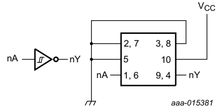
Fig 10. Inverter
