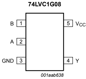
Figure 4. Pin configuration SOT353-1 (TSSOP5) and SOT753 (SC-74A)
