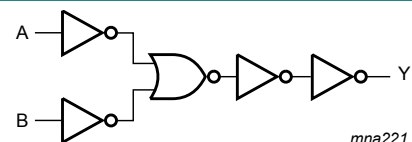
Figure 3. Logic diagram
