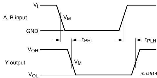
Figure 8. The input A, B to output Y propagation delays
