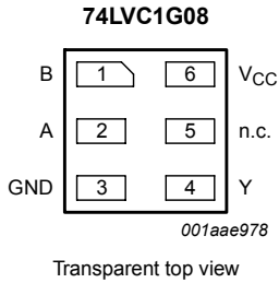
Figure 6. Pin configuration SOT891 (XSON6), SOT1115 (XSON6) and SOT1202 (XSON6)
