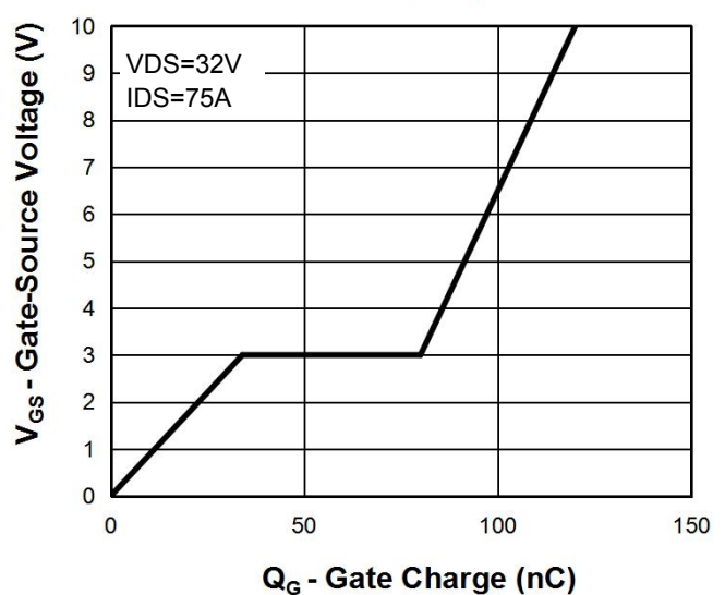
Gate Charge
