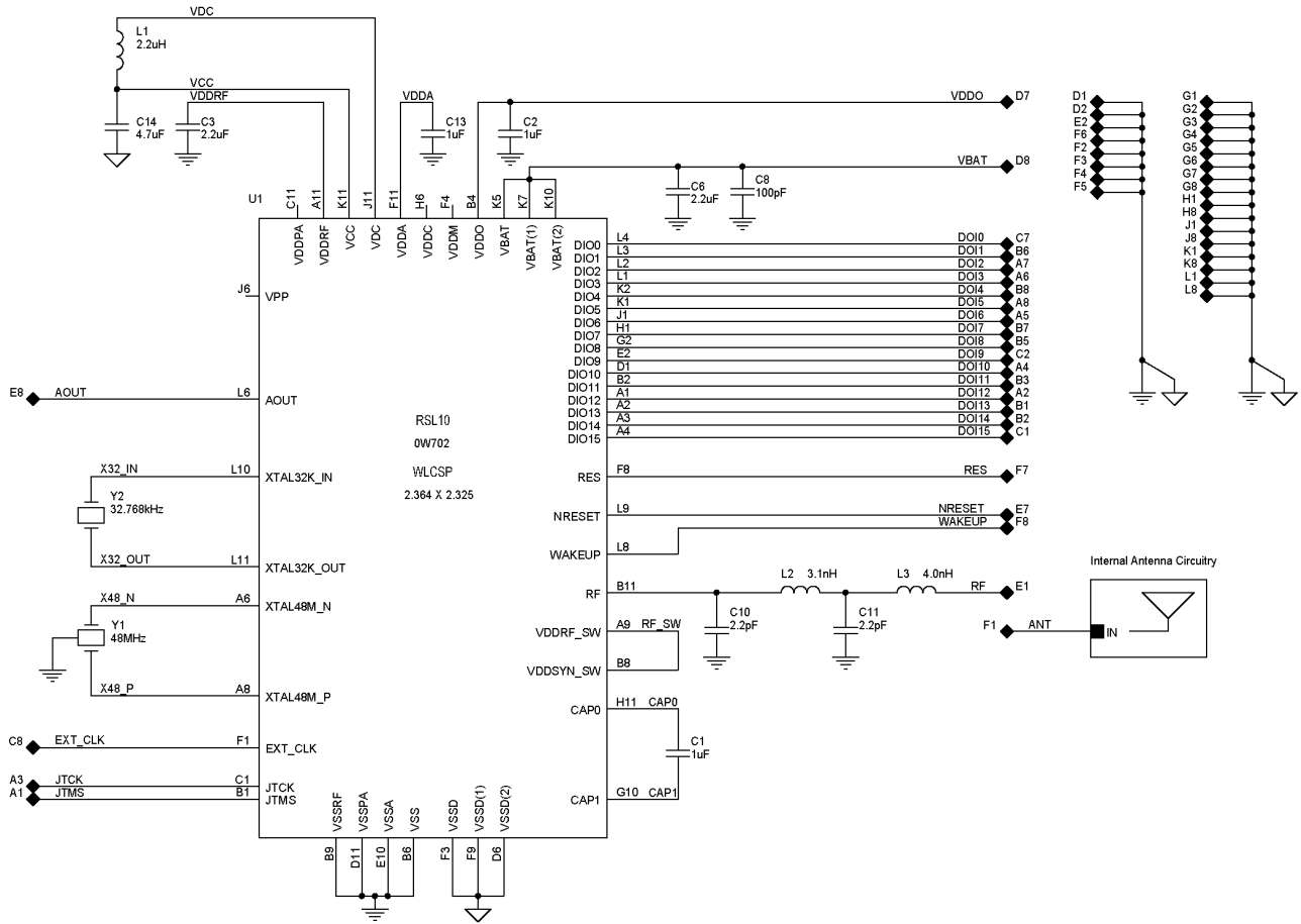
Figure 3. RSL10 Schematic
