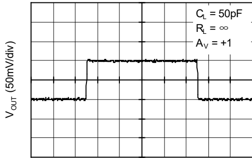
Time (5µs/div)
