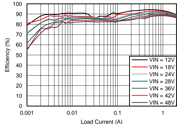
Figure 60. Efficiency
