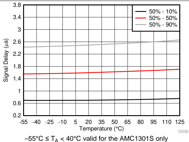
Figure 38. V IN to V OUT Signal Delay vs Temperature
