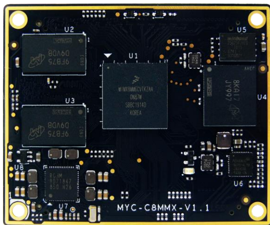
Figure 1-1 MYC-C8MMX CPU Module Top-View
