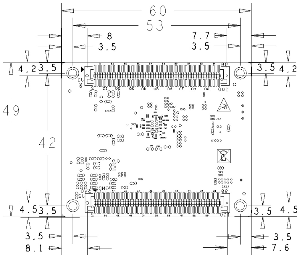
Figure 1-7 MYC-C8MMX Dimensions Chart
