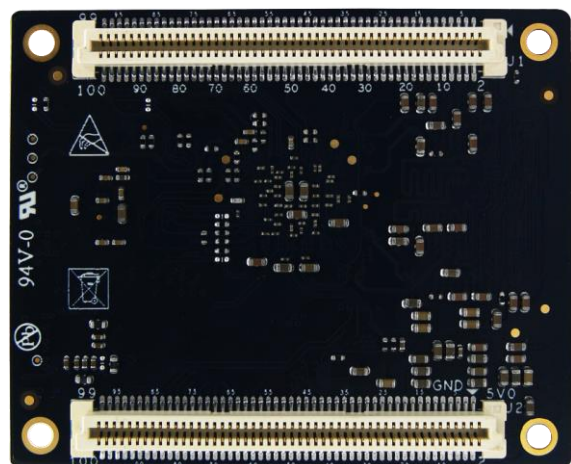
Figure 1-2 MYC-C8MMX CPU Module Bottom-View
