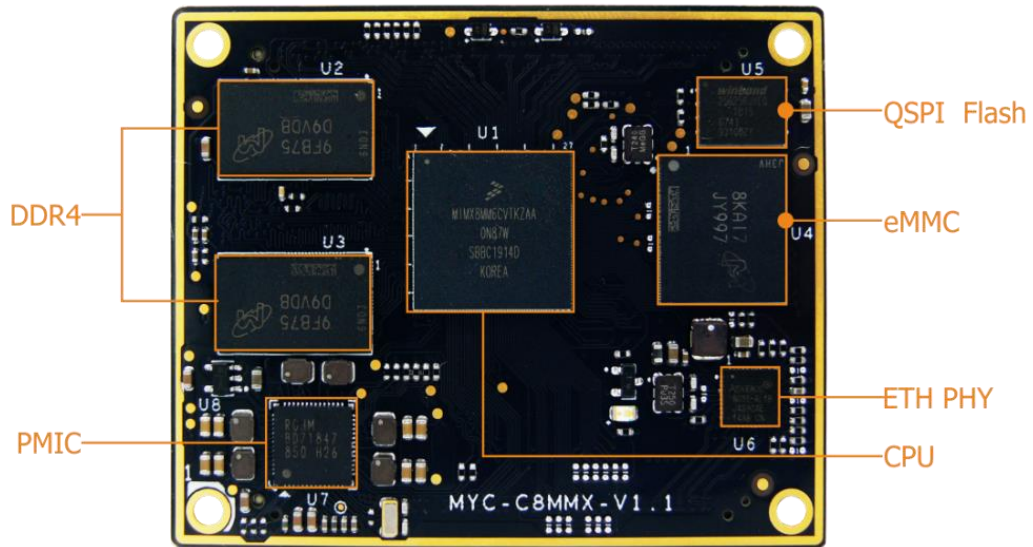
Figure 1-3 MYC-C8MMX CPU Module
