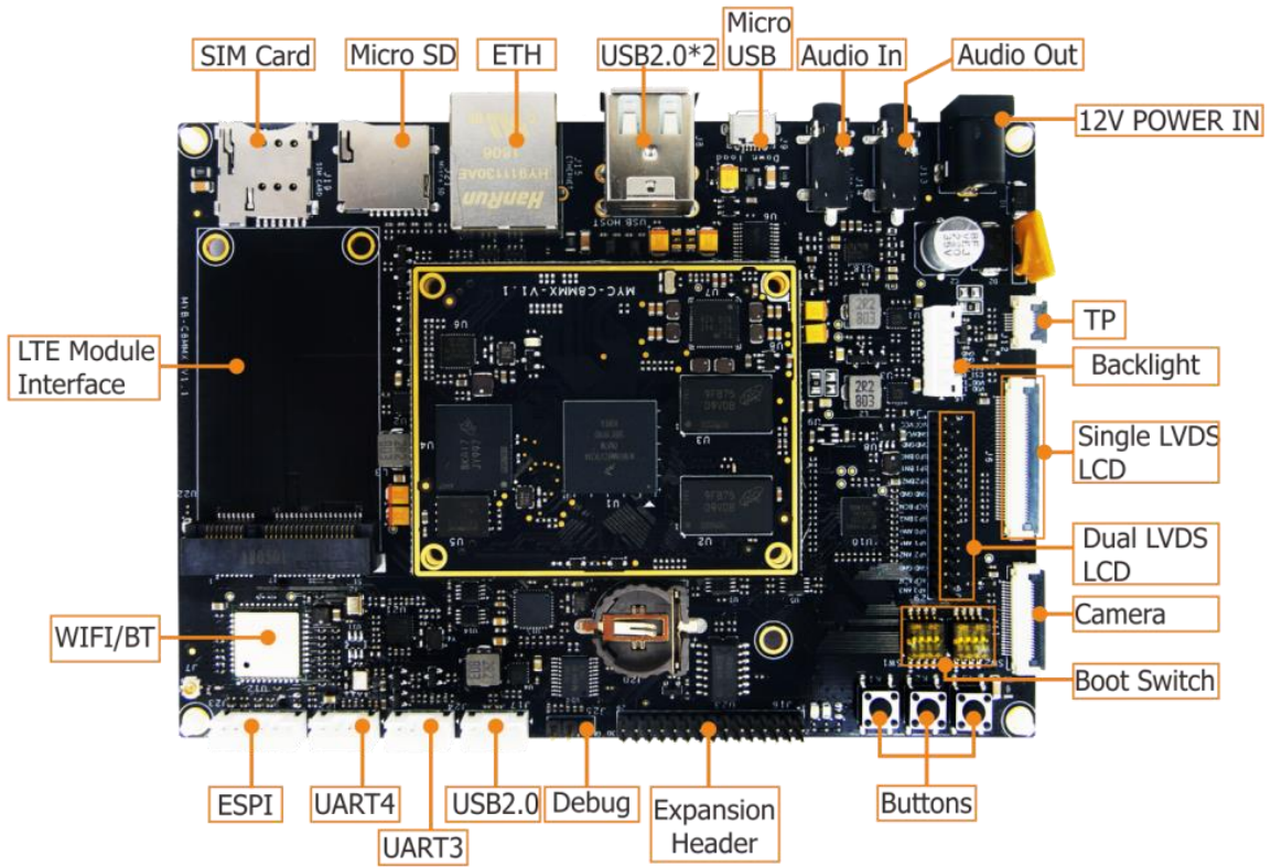
Figure 1-4 MYD-C8MMX Development Board
