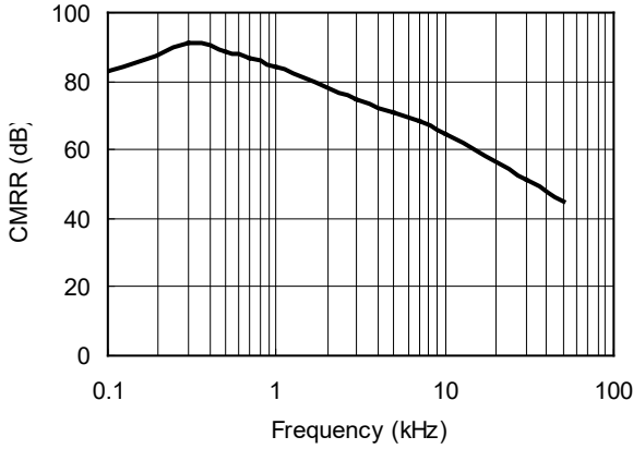
CMRR vs. Frequency at +5V
