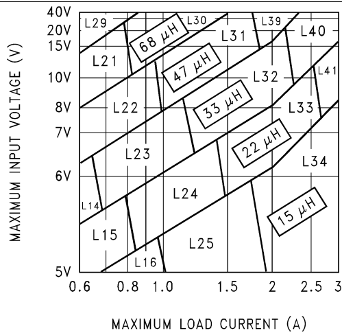
Figure 27. LM2596-3.3
