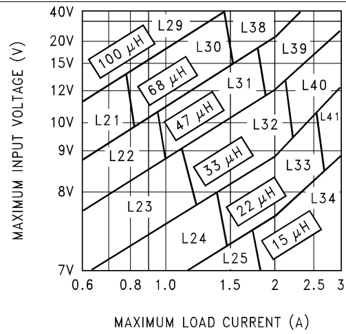
Figure 28. LM2596-5.0
