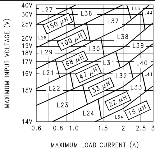
Figure 29. LM2596-12
