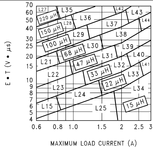
Figure 30. LM2596-ADJ
