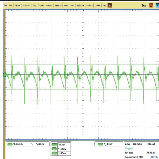
Figure 15. Output Ripple 10 mV/div, 2-μs/div, 20-MHz Bandwidth
