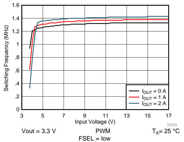
Figure 77. Switching Frequency vs Input Voltage
