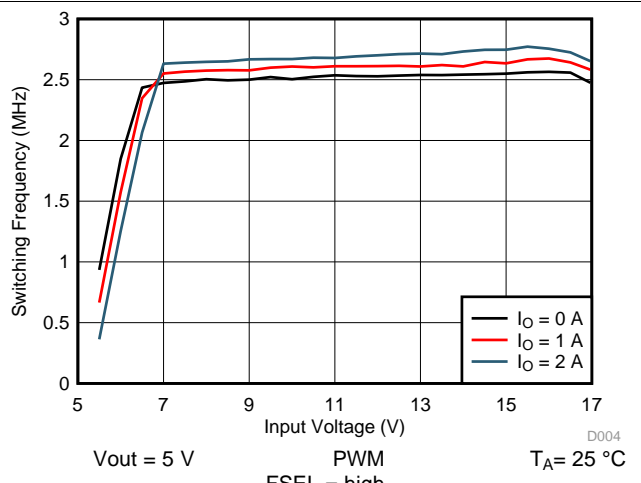
Figure 79. Switching Frequency vs Input Voltage
