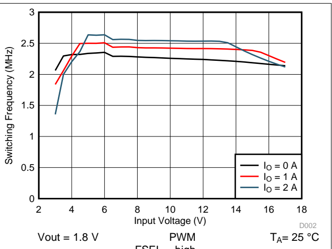
Figure 73. Switching Frequency vs Input Voltage
