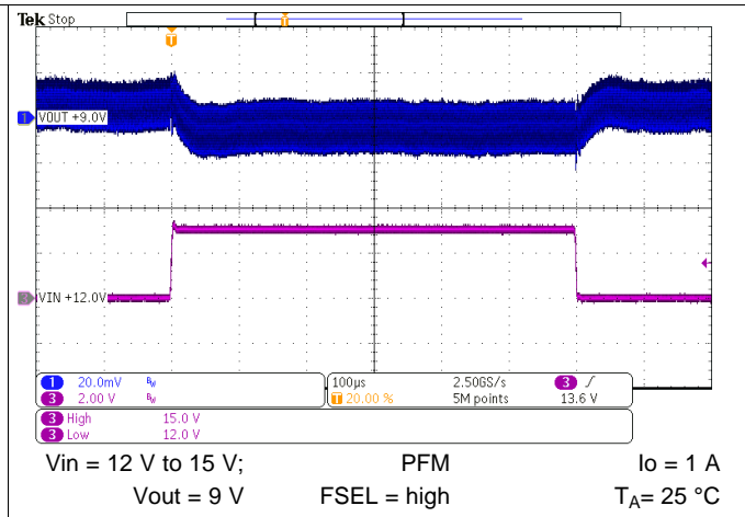
Figure 65. Line Transient Response
