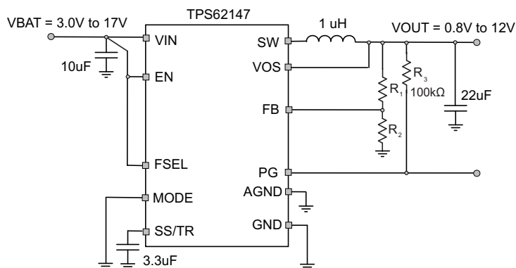
Figure 3. Measurement Setup with FSEL = high
