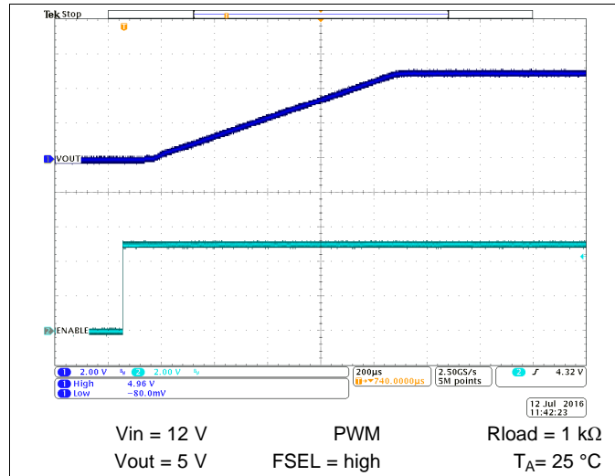
Figure 60. Start-Up Timing
