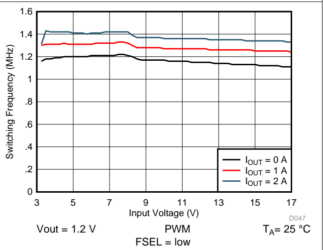
Figure 71. Switching Frequency vs Input Voltage
