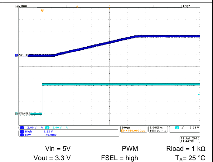
Figure 53. Start-Up Timing
