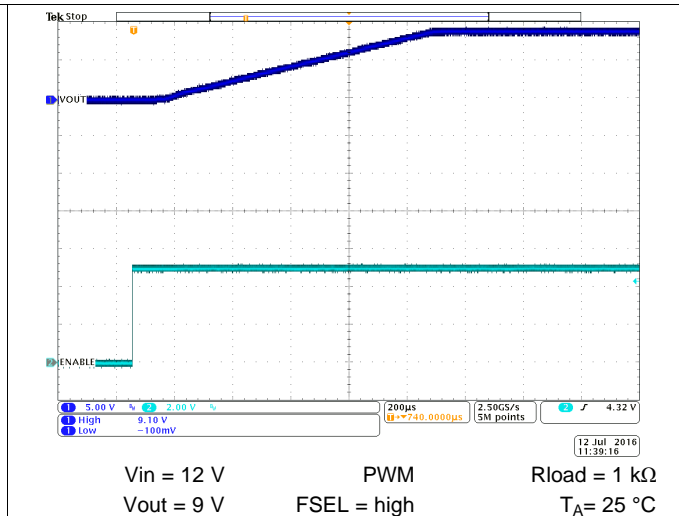
Figure 67. Start-Up Timing
