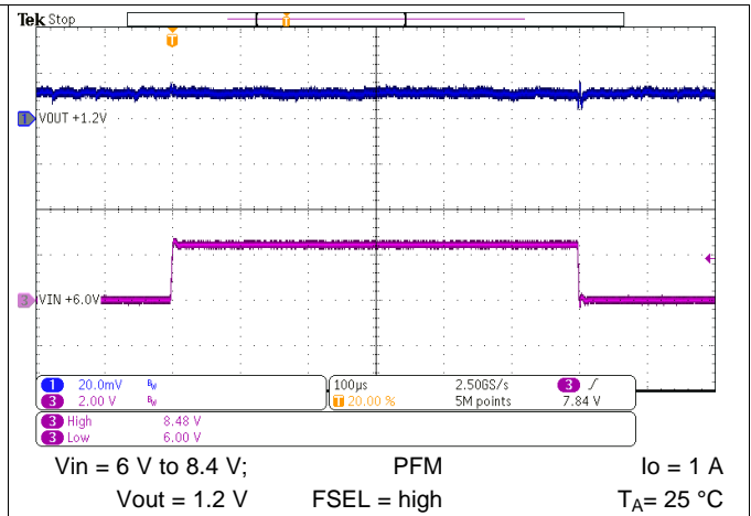
Figure 37. Line Transient Response
