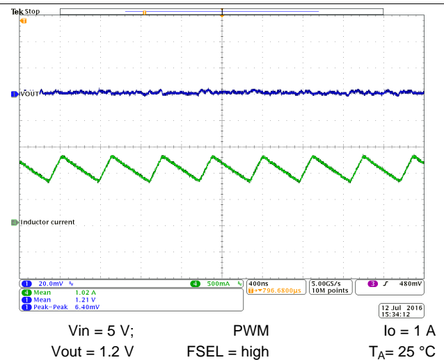
Figure 41. Output Voltage Ripple
