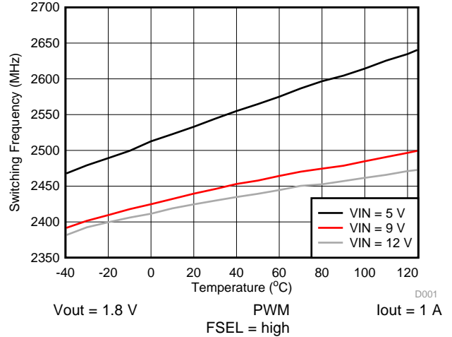
Figure 75. Switching Frequency vs Junction Temperature
