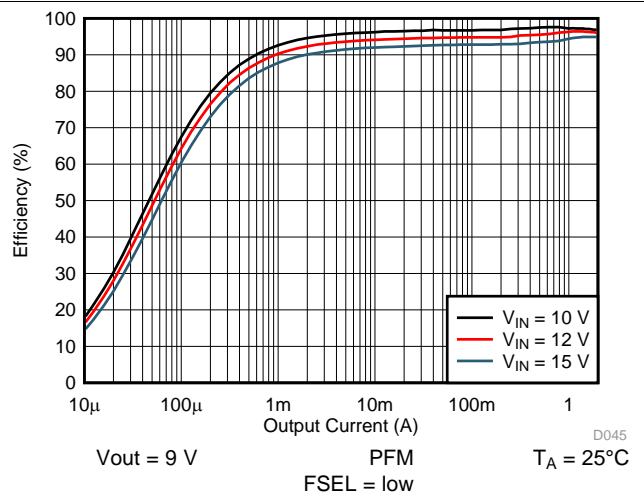
Figure 23. Efficiency vs Output Current
