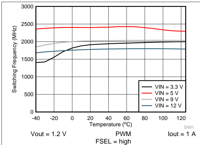
Figure 72. Switching Frequency vs Junction Temperature
