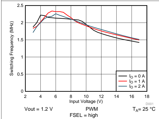
Figure 70. Switching Frequency vs Input Voltage
