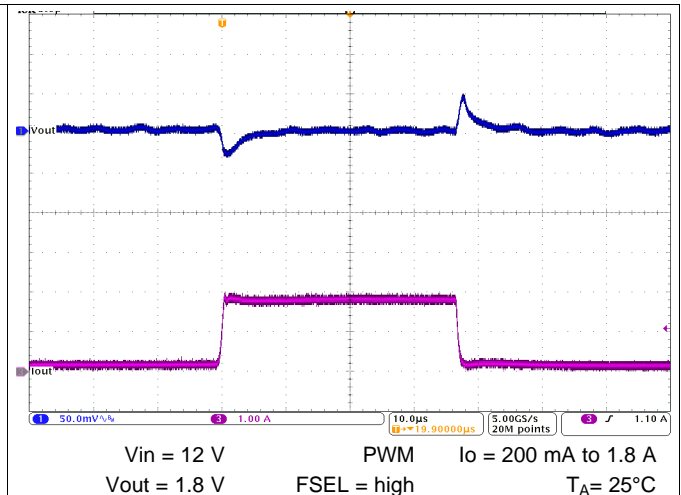
Figure 43. Load Transient Response
