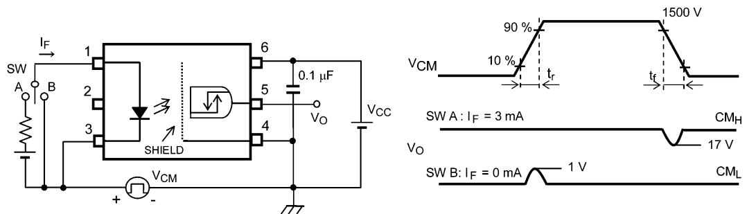
Fig. 12.1.8 Common-Mode Transient Immunity Test Circuit and Waveform
