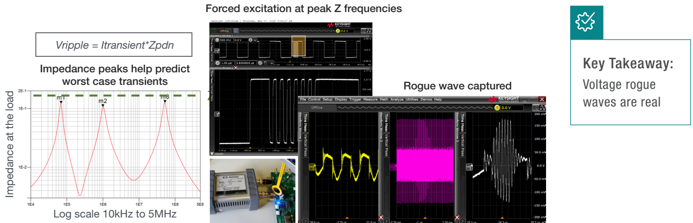
Figure 4. Multiple impedance peaks in the frequency domain result in power rail ripple and can be a source of rogue voltage waves
