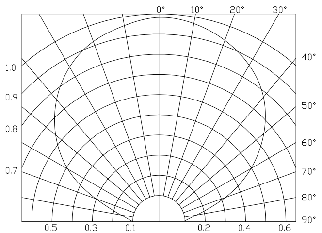
Radiation Diagram
