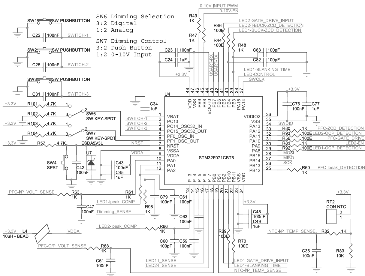
Figure 5: STEVAL-LLL004V1 schematic - STM32 microcontroller
