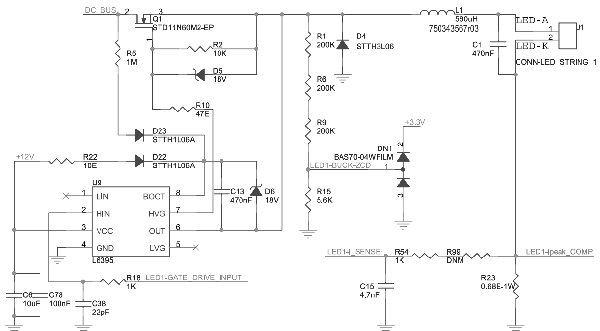
Figure 3: STEVAL-LLL004V1 schematic - buck converter
