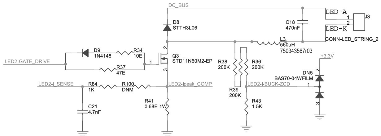
Figure 2: STEVAL-LLL004V1 schematic - inverse buck converter
