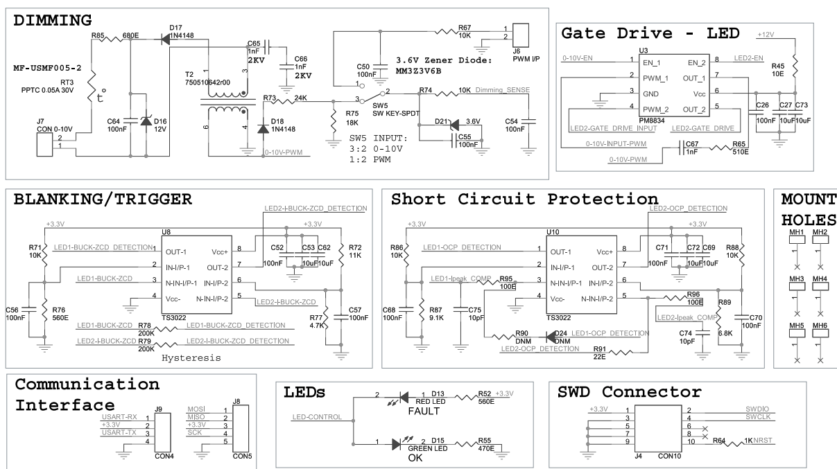
Figure 6: STEVAL-LLL004V1 schematic - miscellaneous
