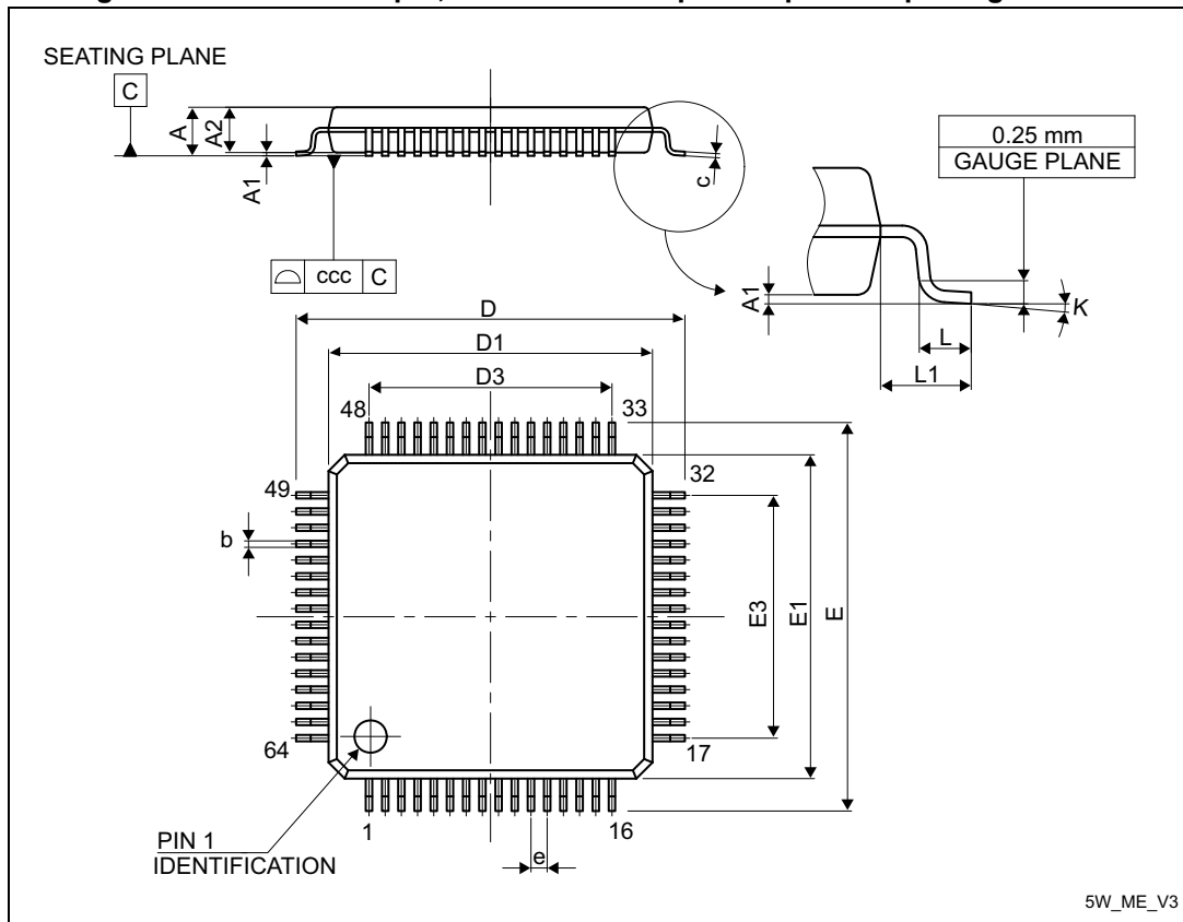
Figure 82. LQFP64 - 64-pin, 10 x 10 mm low-profile quad flat package outline
