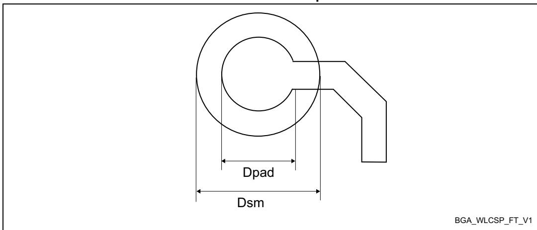
Figure 89. WLCSP - 81 balls, 4.36 x 4.07 mm, 0.4 mm pitch, wafer level chip scale recommended footprint
