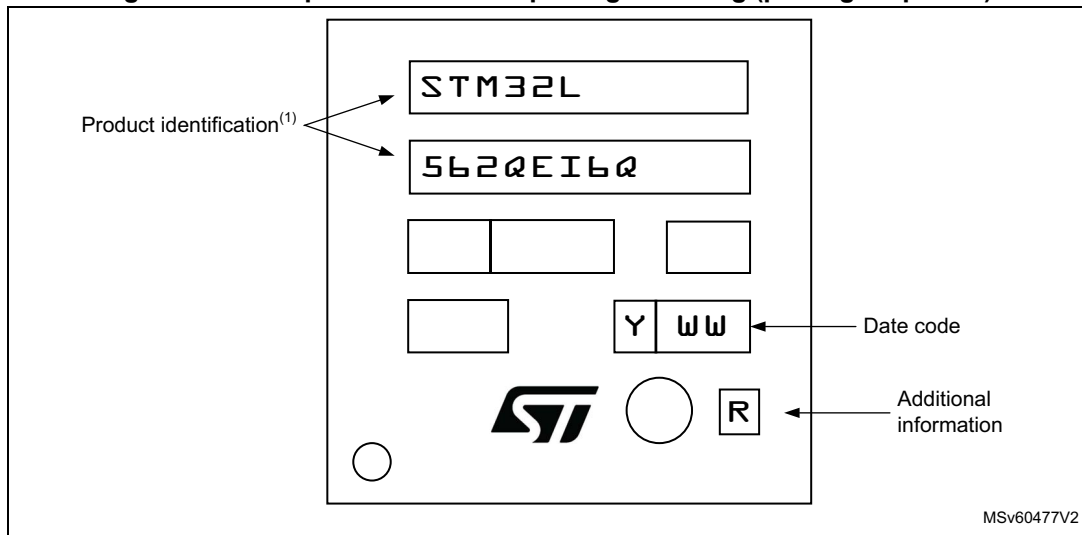
Figure 87. Example of UFBGA132 package marking (package top view)
