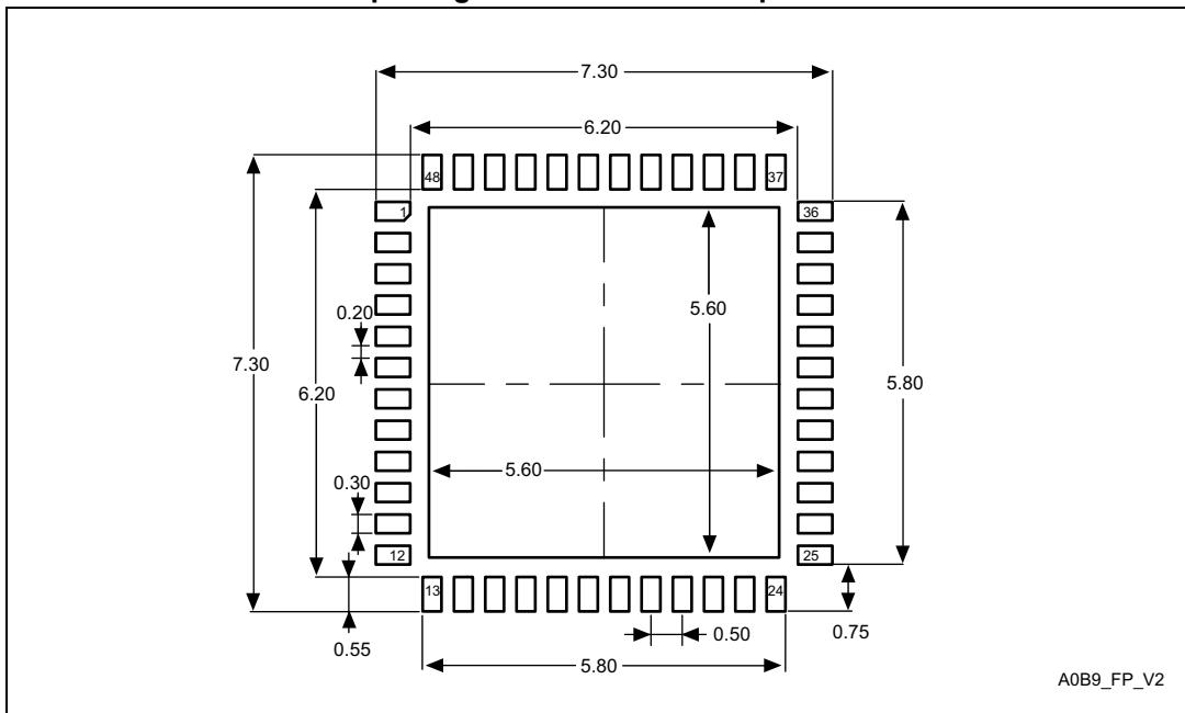
Figure 77. UFQFPN48 - 48-lead, 7x7 mm, 0.5 mm pitch, ultra thin fine pitch quad flat package recommended footprint
