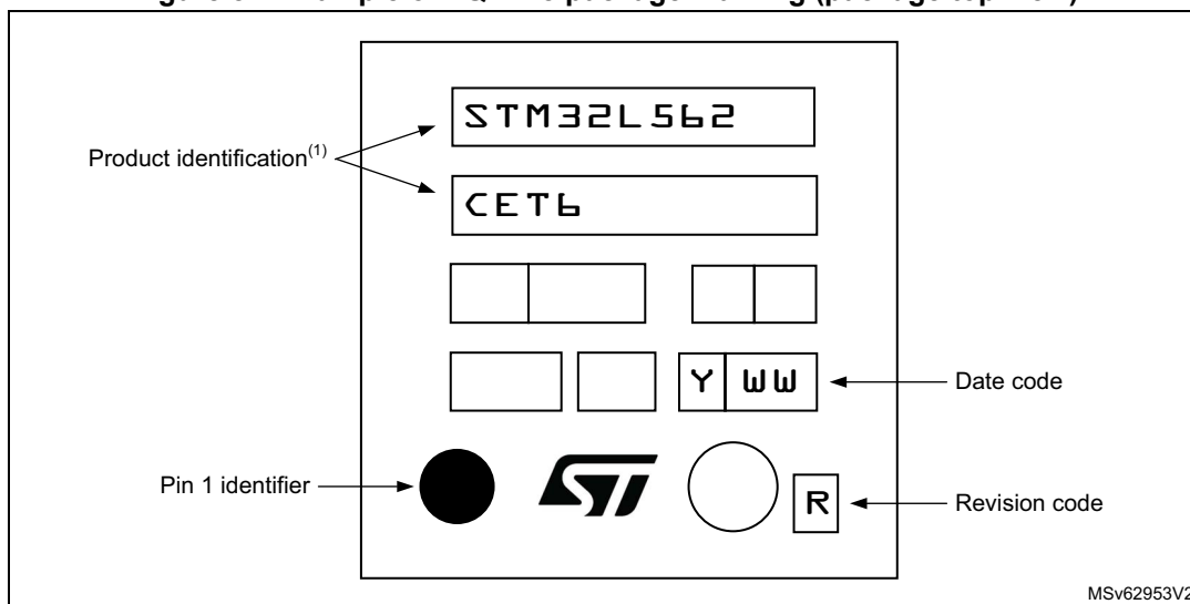
Figure 81. Example of LQFP48 package marking (package top view)
