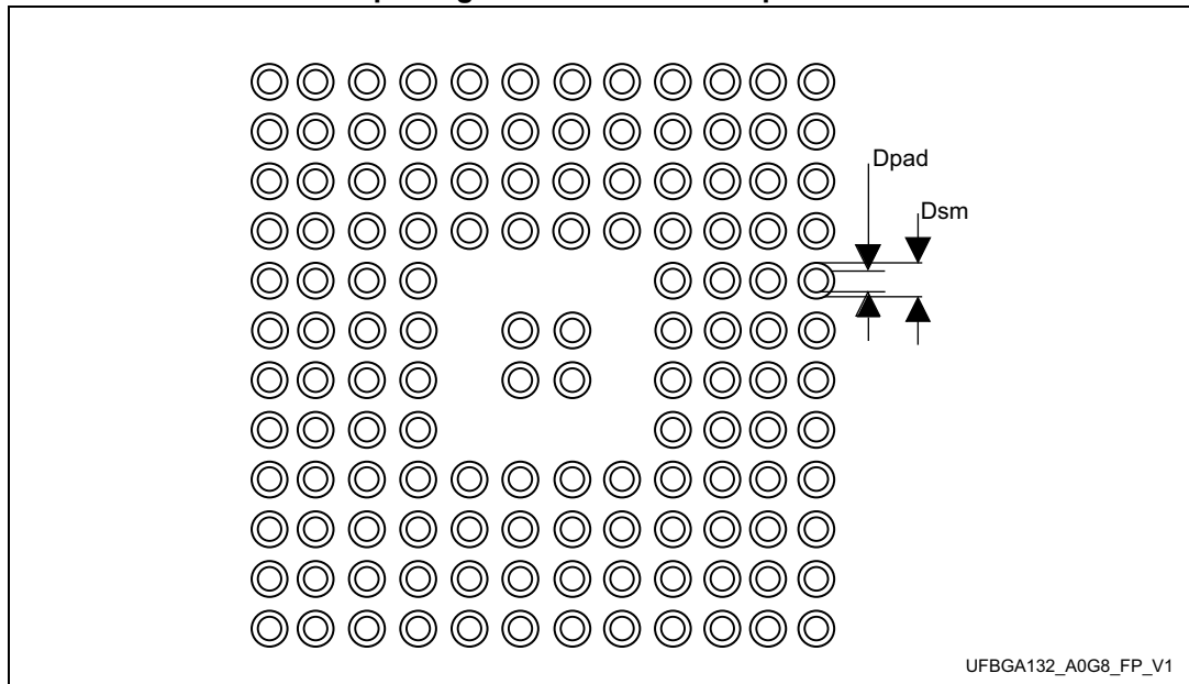
Figure 86. UFBGA132 - 132-ball, 7 x 7 mm ultra thin fine pitch ball grid array package recommended footprint
