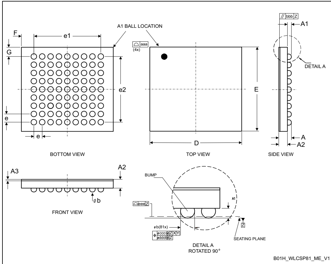
Figure 88. WLCSP - 81 balls, 4.36 x 4.07 mm, 0.4 mm pitch, wafer level chip scale package outline
