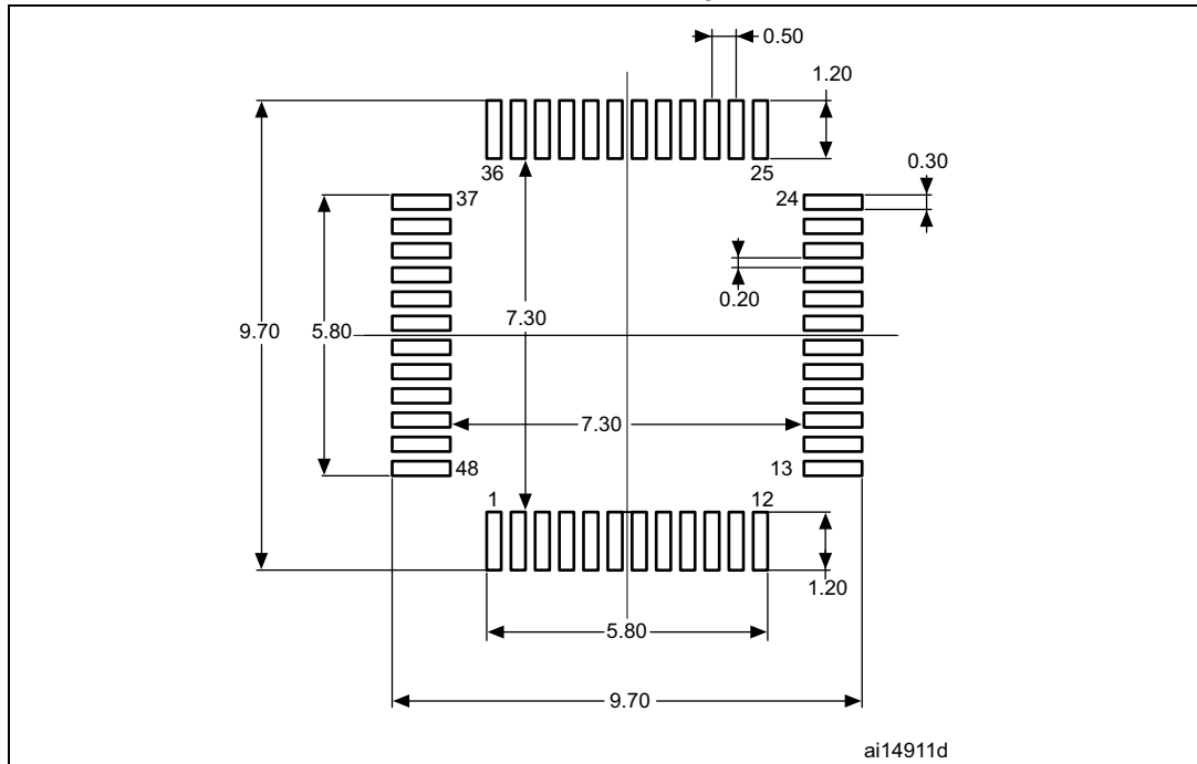
Figure 80. LQFP48 - 48-pin, 7 x 7 mm low-profile quad flat package recommended footprint
