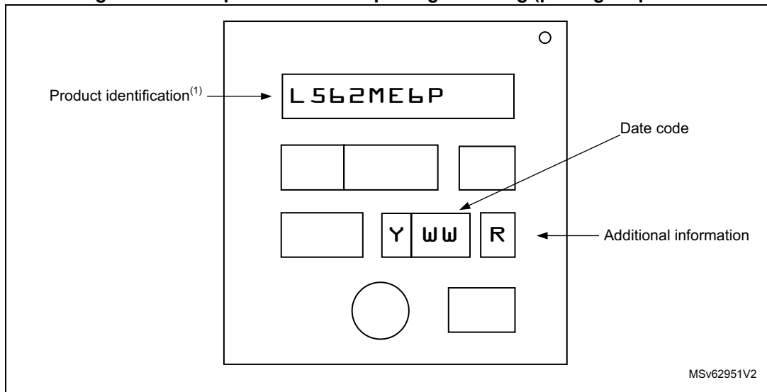
Figure 90. Example of WLCSP81 package marking (package top view)
