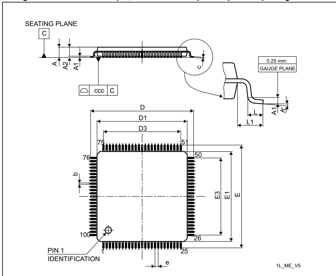
Figure 91. LQFP100 - 100-pin, 14 x 14 mm low-profile quad flat package outline
