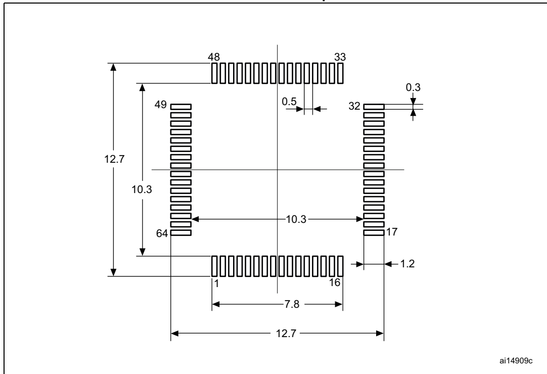
Figure 83. LQFP64 - 64-pin, 10 x 10 mm low-profile quad flat package recommended footprint
