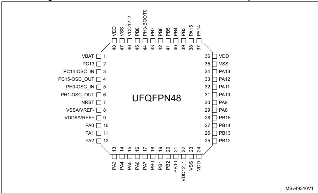
Figure 13. STM32L562xxxxP UFQFPN48 external SMPS pinout (1)
