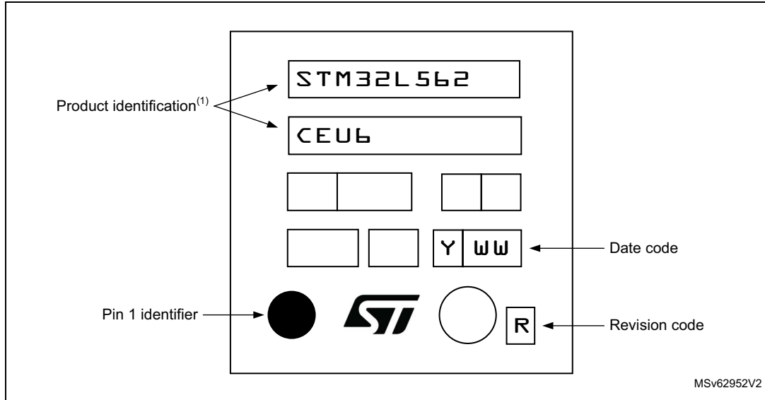
Figure 78. Example of UFQFPN48 package marking (package top view)
