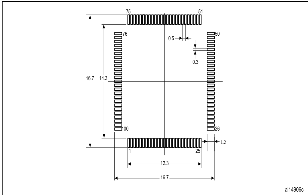
Figure 92. LQFP100 - 100-pin, 14 x 14 mm low-profile quad flat recommended footprint
