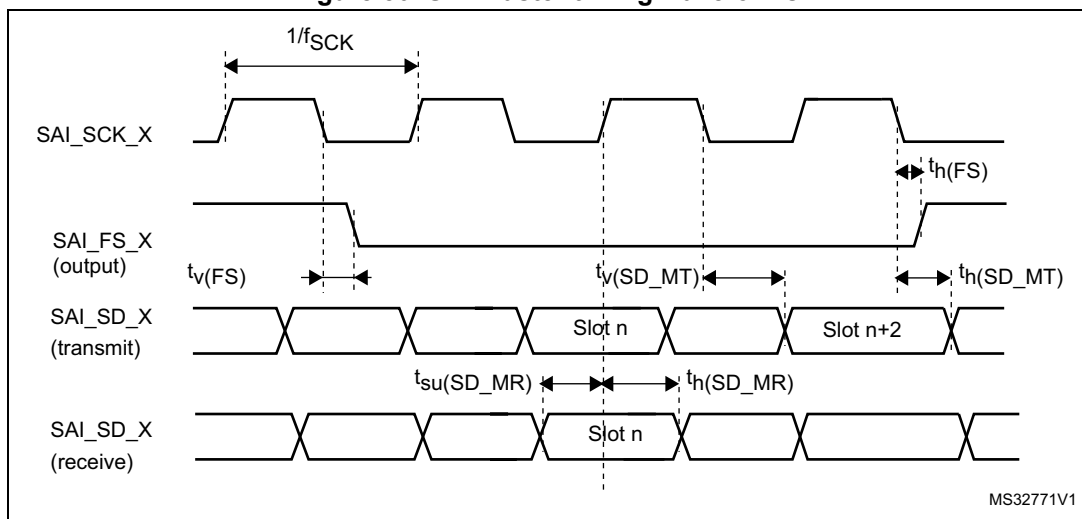
Figure 50. SAI master timing waveforms
