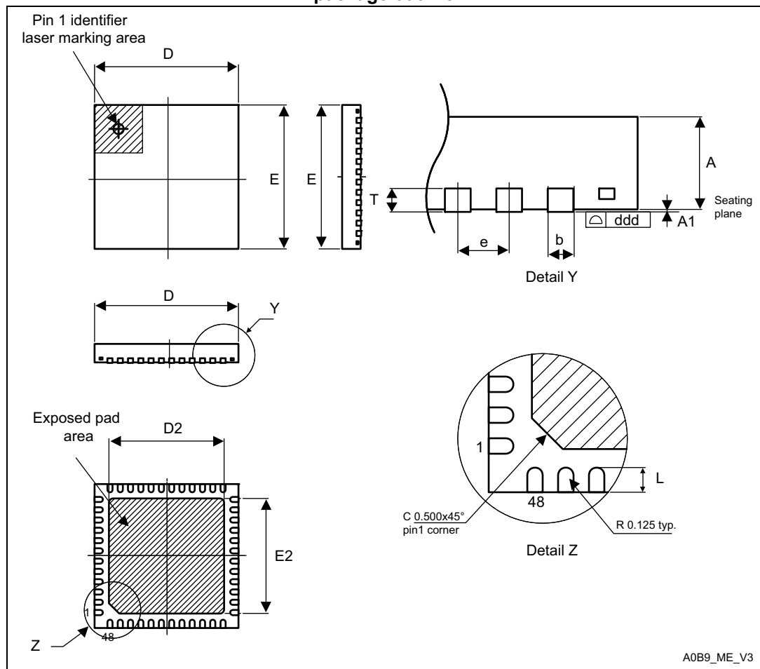
Figure 76. UFQFPN48 - 48-lead, 7x7 mm, 0.5 mm pitch, ultra thin fine pitch quad flat package outline
