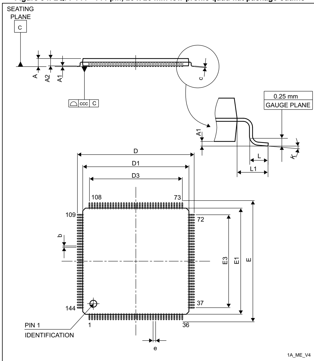
Figure 94. LQFP144 - 144-pin, 20 x 20 mm low-profile quad flat package outline
