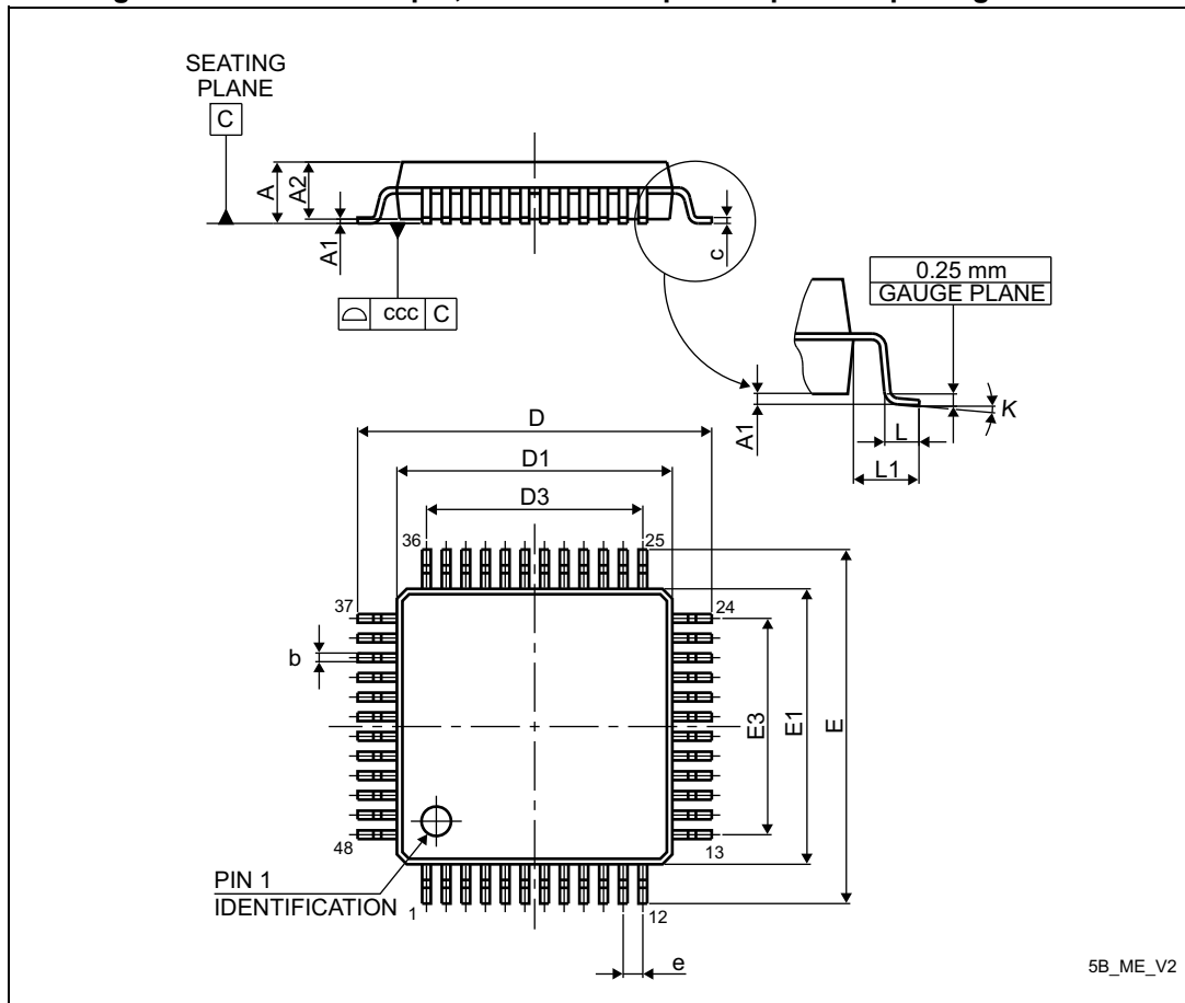
Figure 79. LQFP48 - 48-pin, 7 x 7 mm low-profile quad flat package outline
