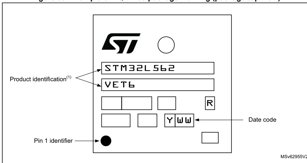
Figure 93. Example of LQFP100 package marking (package top view)
