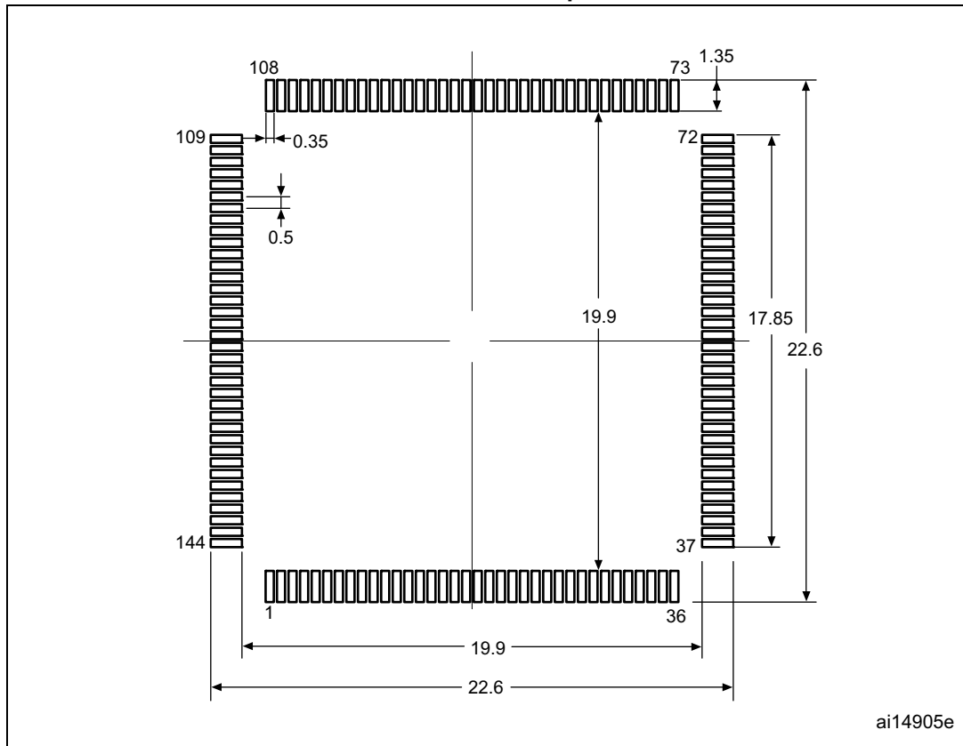
Figure 95. LQFP144 - 144-pin, 20 x 20 mm low-profile quad flat package recommended footprint
