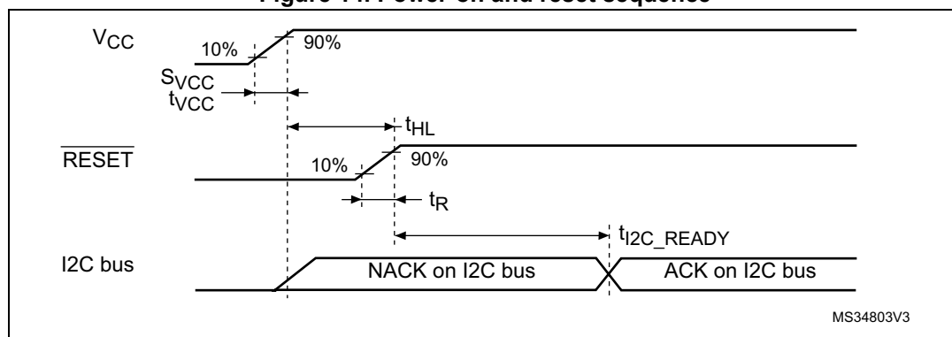
Figure 15. Warm reset sequence
