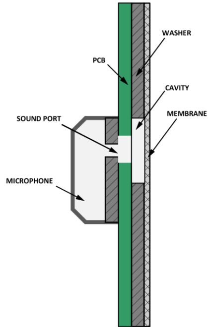
Figure 5. Cross-Section of Experimental Seal Structure
