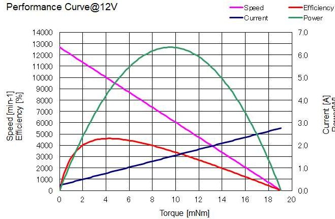
Performance Curve@12V
