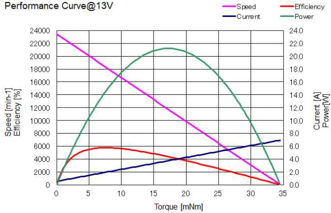
Performance Curve@13V
