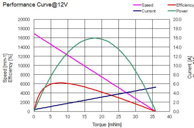
Performance Curve@12V
