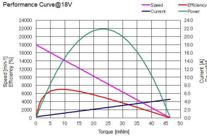
Performance Curve@18V
