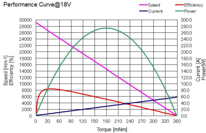
Performance Curve@18V
