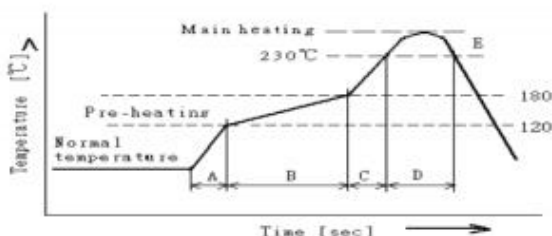
Temperature Profile
