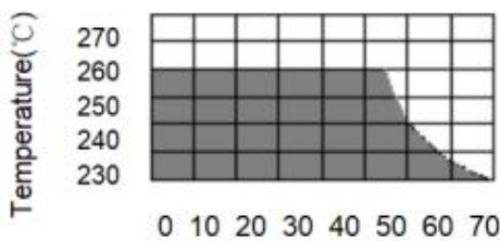
Temperature Profile
