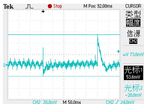
14. Load transient response (IL=0-350-0mA)
