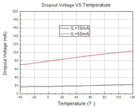
9. Dropout Voltage VS Temperature
