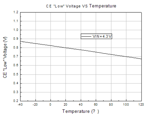
11. CE "Low" Voltage VS Temperature
