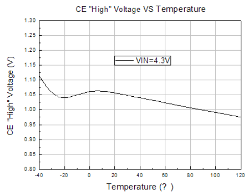
10. CE "High" Voltage VS Temperature
