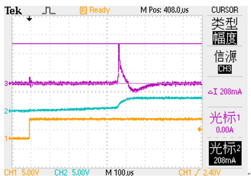
19. Inrush Current
