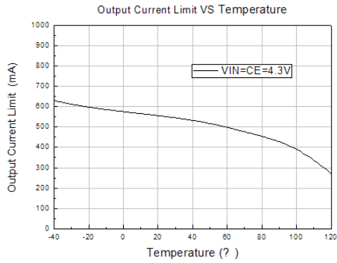
7. Output Current Limit VS Temperature
