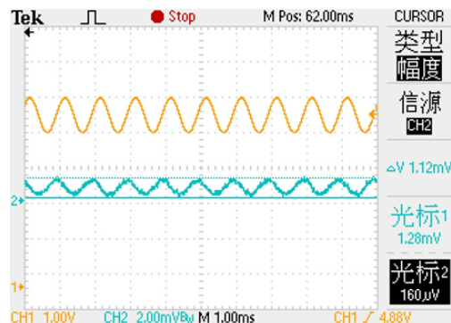
16. Ripple-Rejection (IL=50mA, Vpp=1V, F=1KHZ)
