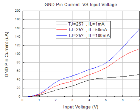
4. GND Pin Current VS Input Voltage
