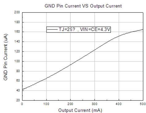
5. GND Pin Current VS Output Current
