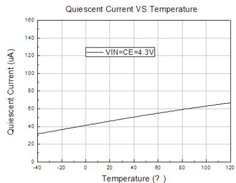
6. Quiescent Current VS Temperature
