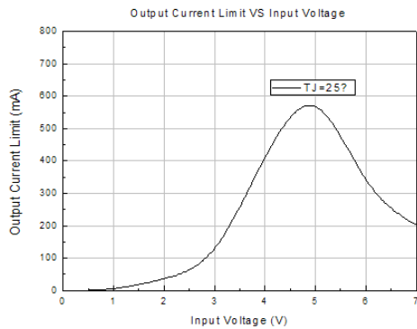
3. Output Current Limit VS Input Voltage
