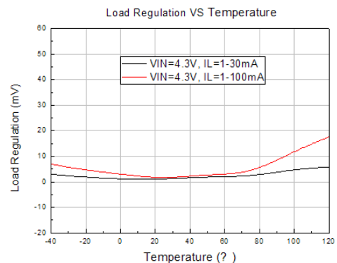
12. Load Regulation VS Temperature
