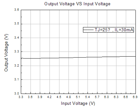
2. Output Voltage VS Input Voltage
