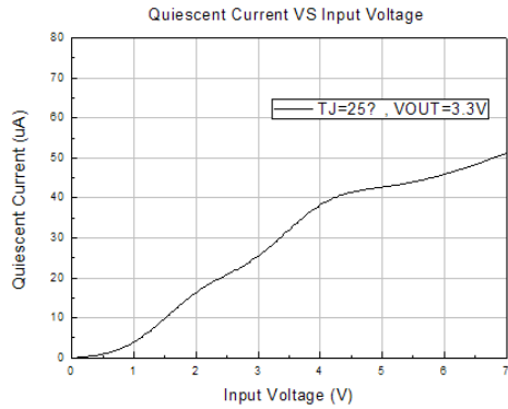
1. Quiescent Current VS Input Voltage
