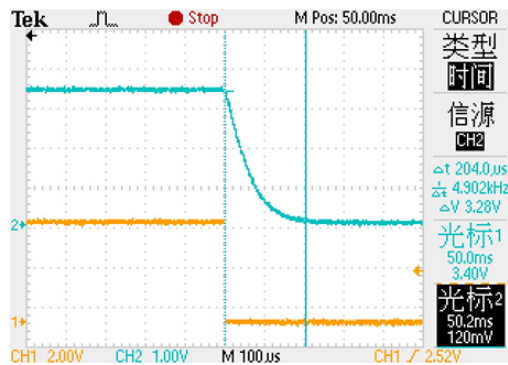
18. CE Turn-off Time
