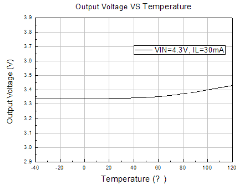
8. Output Voltage VS Temperature
