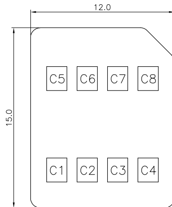
SIM CARD PAD LAYOUT
