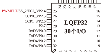
LQFP32 (9x9mm)
