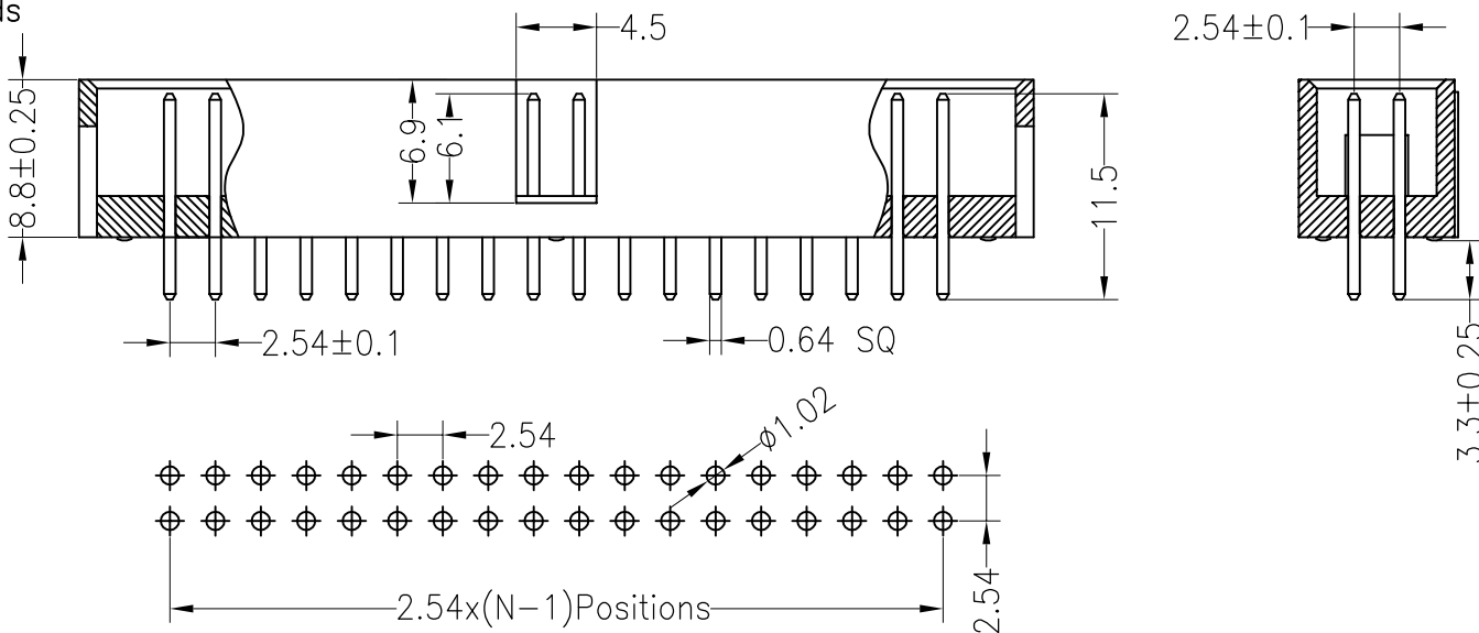
Recommended P.C.B Layout(Top Side) (PCB BOARD TOLERANCE±0.05)
